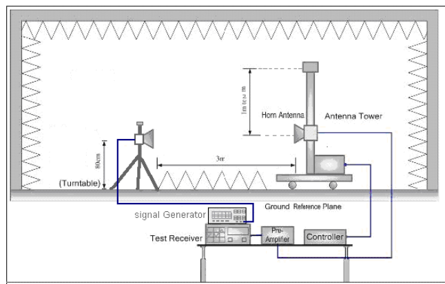
Figure 4. above 1GHz
