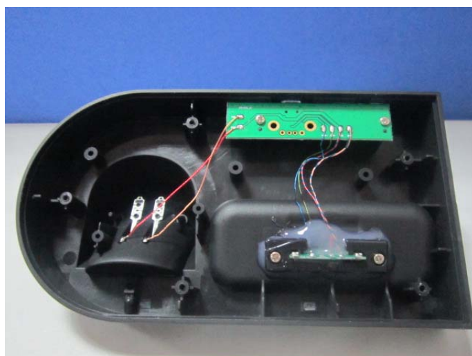
Internal Photos-Charging base
