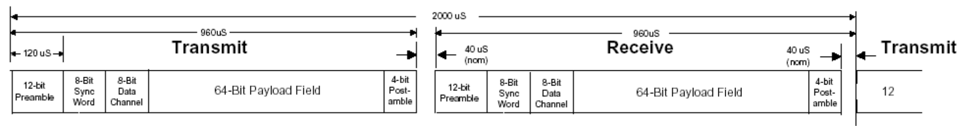
TDD FRAME FORMAT
