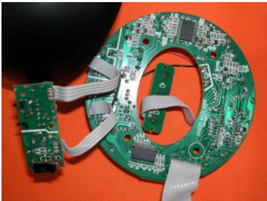
Base Main PCB solder side (View 1)
