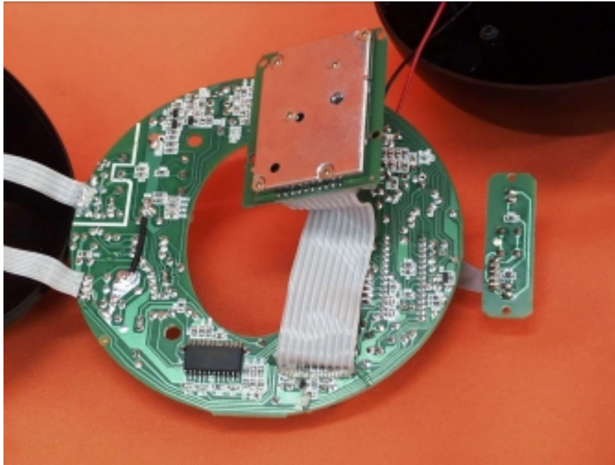
Base Oscillator PCB comp side
