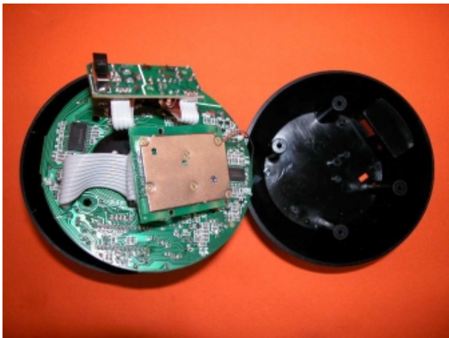
Base assembly (View 2)
