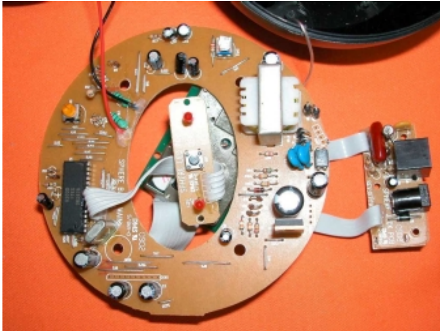
Base Main PCB comp side
