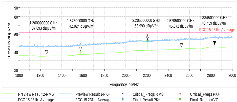
Plot # 3 Radiated Emissions: 1GHz - 3 GHz
