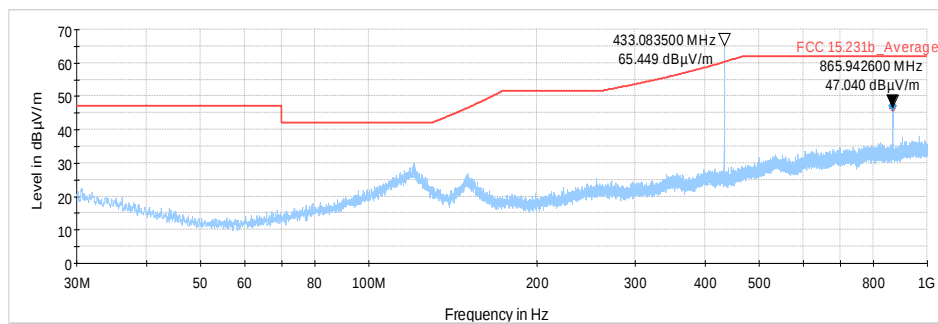
Plot # 6 Radiated Emissions: 30 MHz – 1GHz
