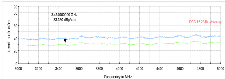
Plot # 4 Radiated Emissions: 3 GHz - 5 GHz
