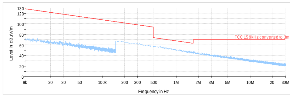
Plot # 5 Radiated Emissions: 9 KHz – 30 MHz
