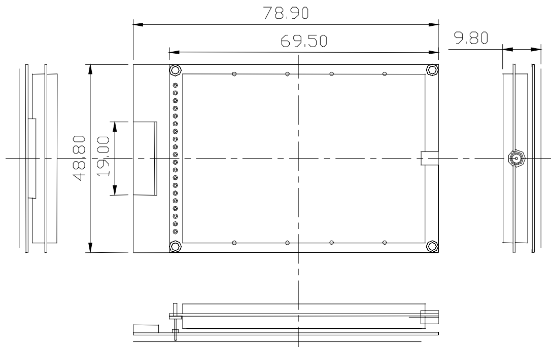
Figure 2-1 Mechanical size of the USWD500 (unit = mm)
