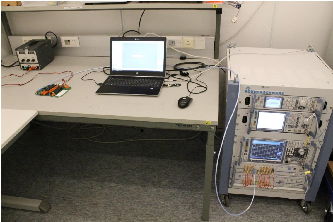
Photograph 6. FCC Conducted measurement
