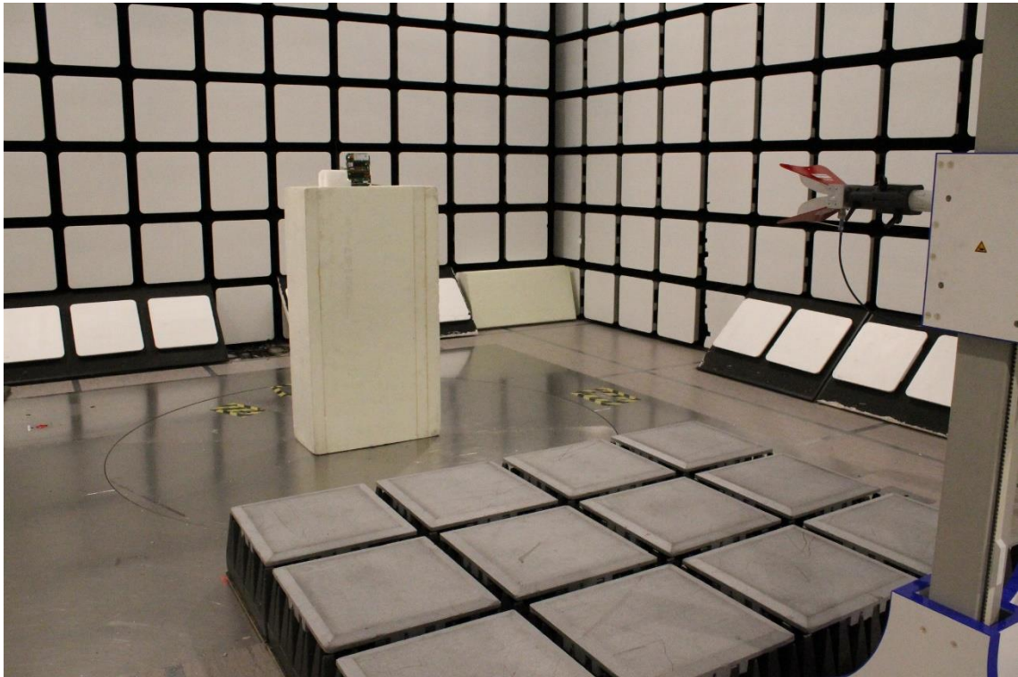
Photograph 3. Radiated Spurious Emissions 1 GHz – 18 GHz
