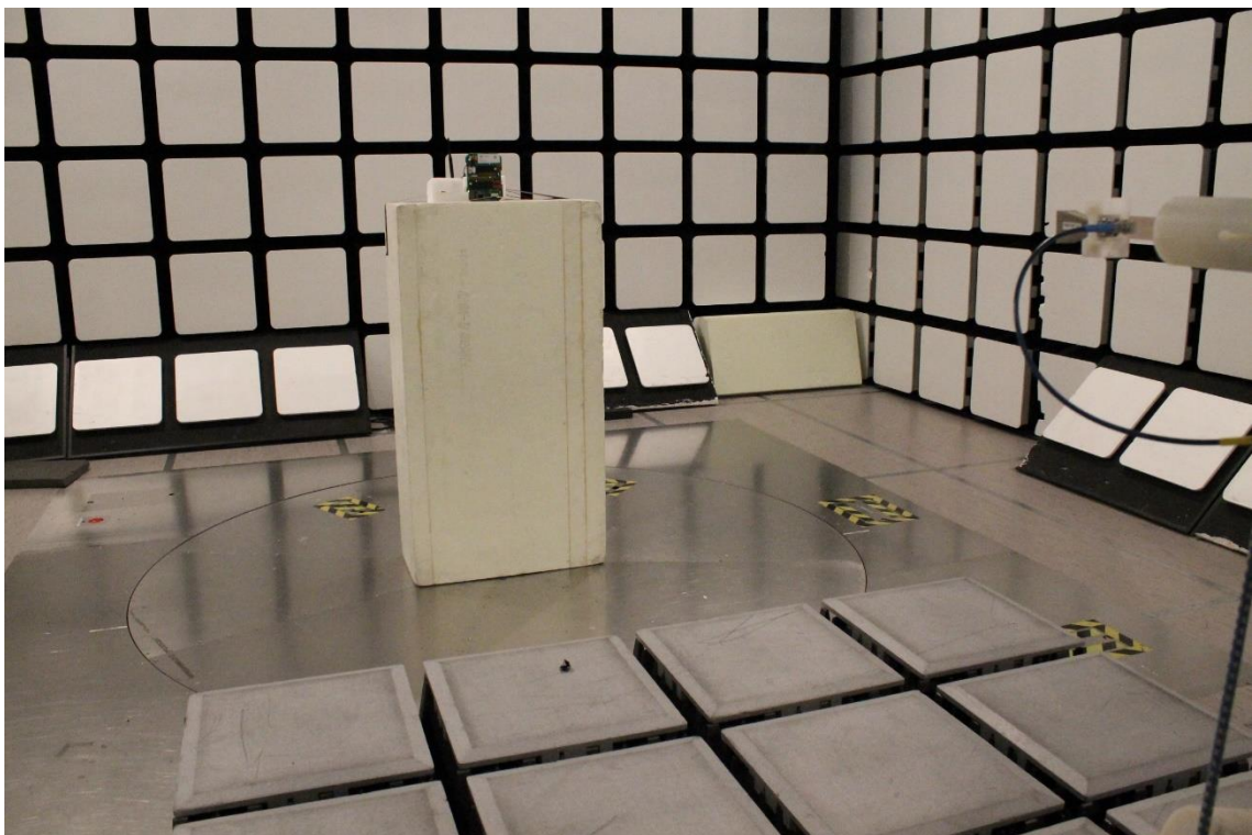
Photograph 4. Radiated Spurious Emissions 18 GHz – 26.5 GHz
