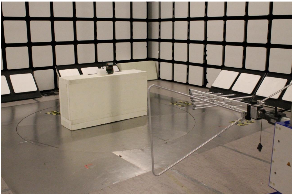
Photograph 2. Radiated Spurious Emissions 30 MHz – 1000 MHz
