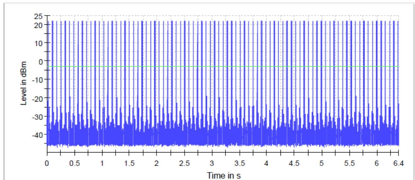
Figure 36: Time of channel occupancy MID channel
