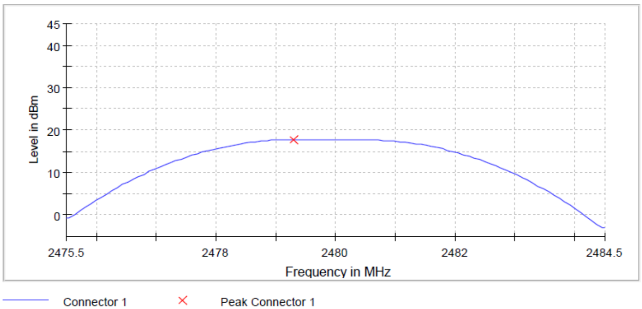
Figure 4: Conducted power, Channel HIGH
