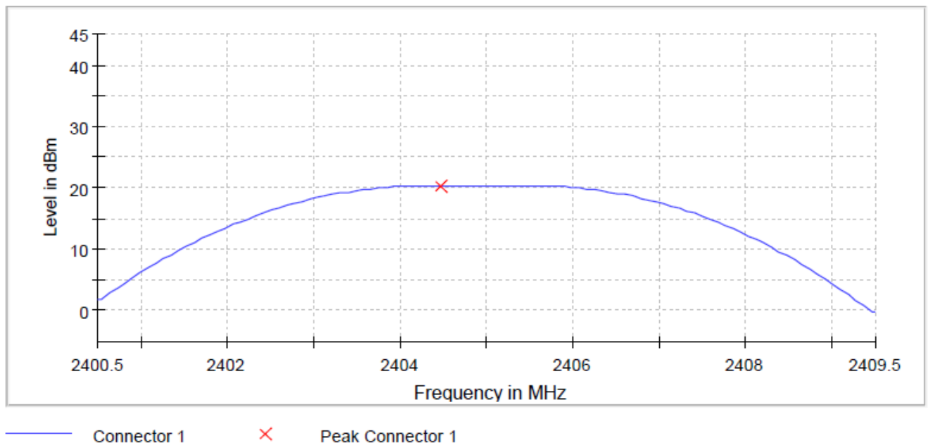
Figure 2: Conducted power, Channel LOW
