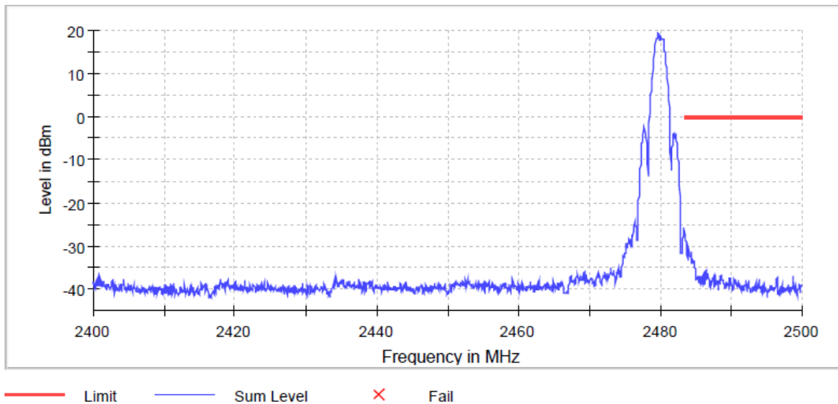
Figure 22: Upper Band Edge
