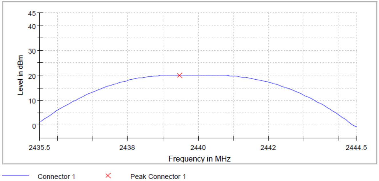
Figure 3: Conducted power, Channel MID
