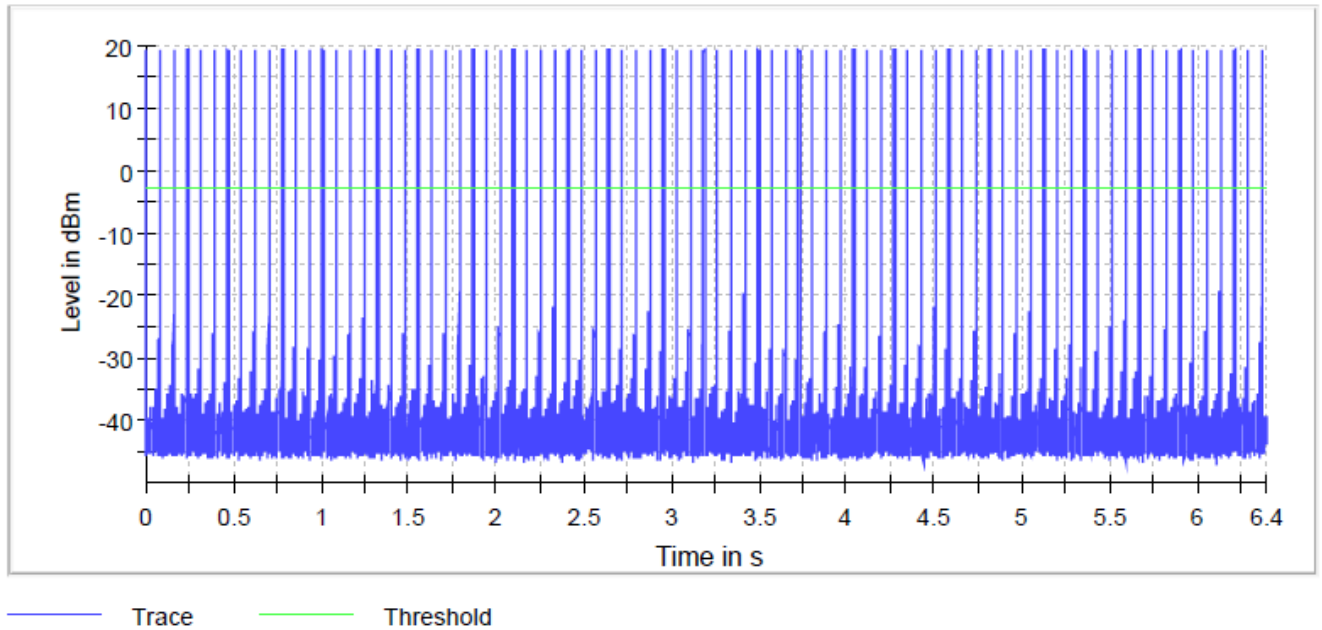
Figure 37: Time of channel occupancy HIGH channel
