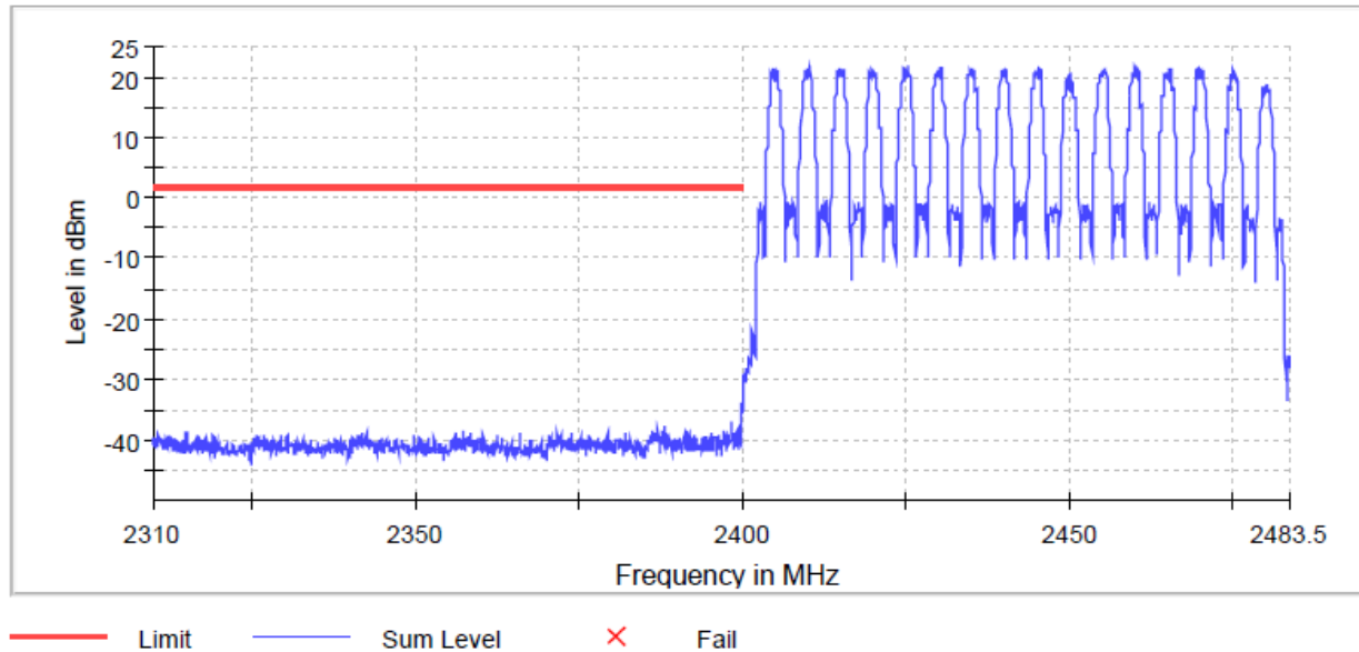
Figure 23: Lower Band Edge, hopping mode
