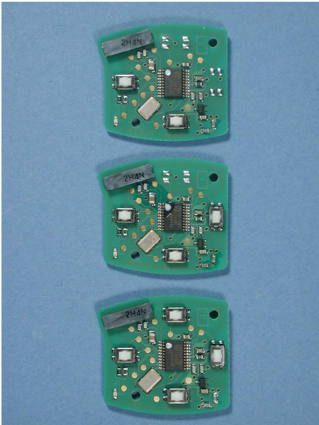
S0084-A PCB component side (all variants)
