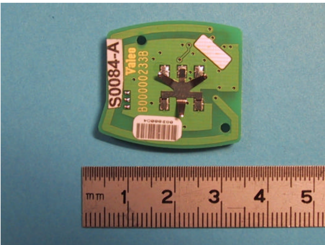
Transmitter S0084A PCB side 2 version 2 buttons
