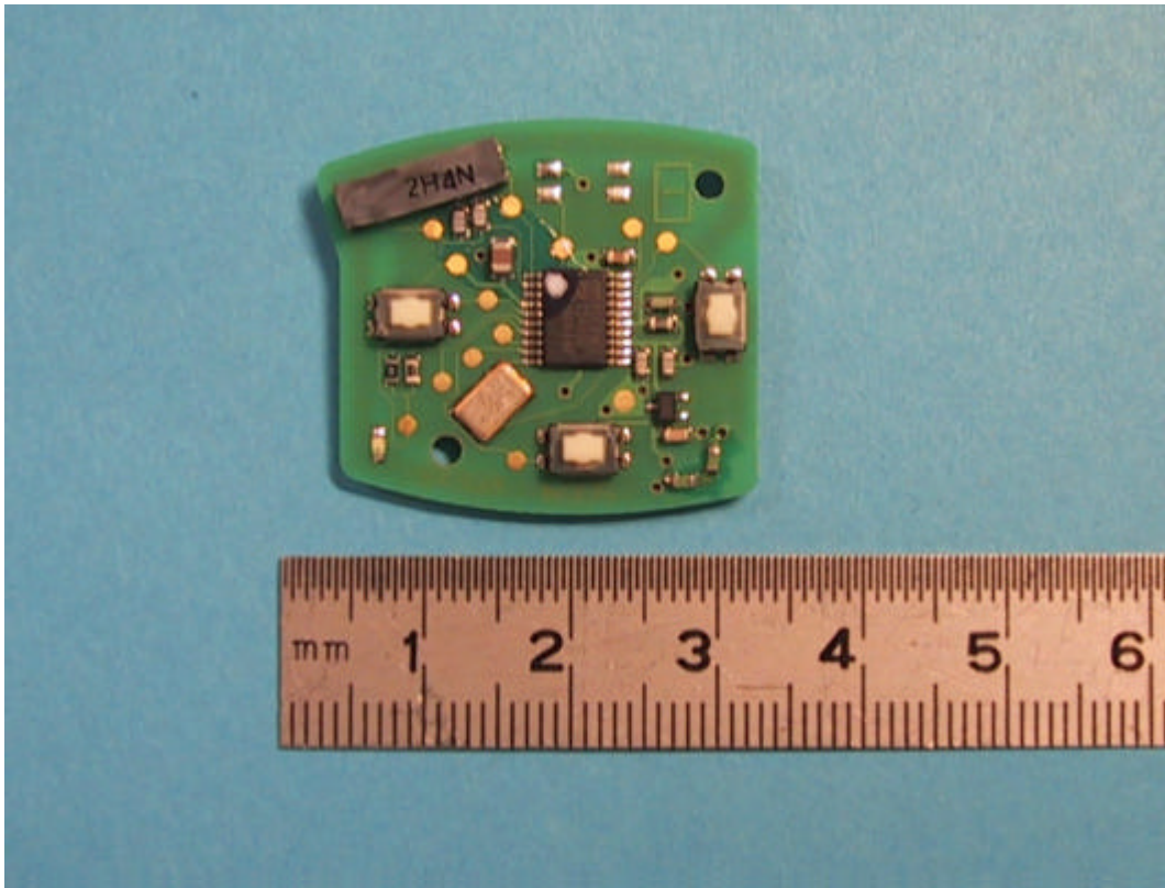
Transmitter S0084A PCB side 2 version 3 buttons
