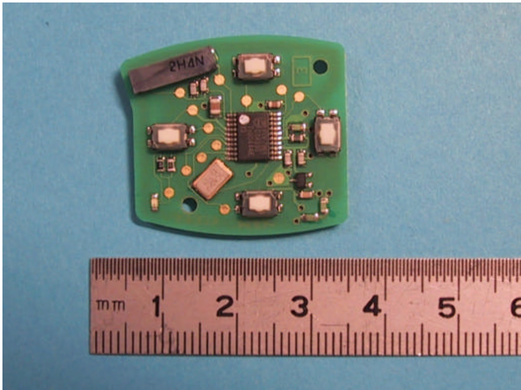
Transmitter S0084A PCB side 1 version 4 buttons
