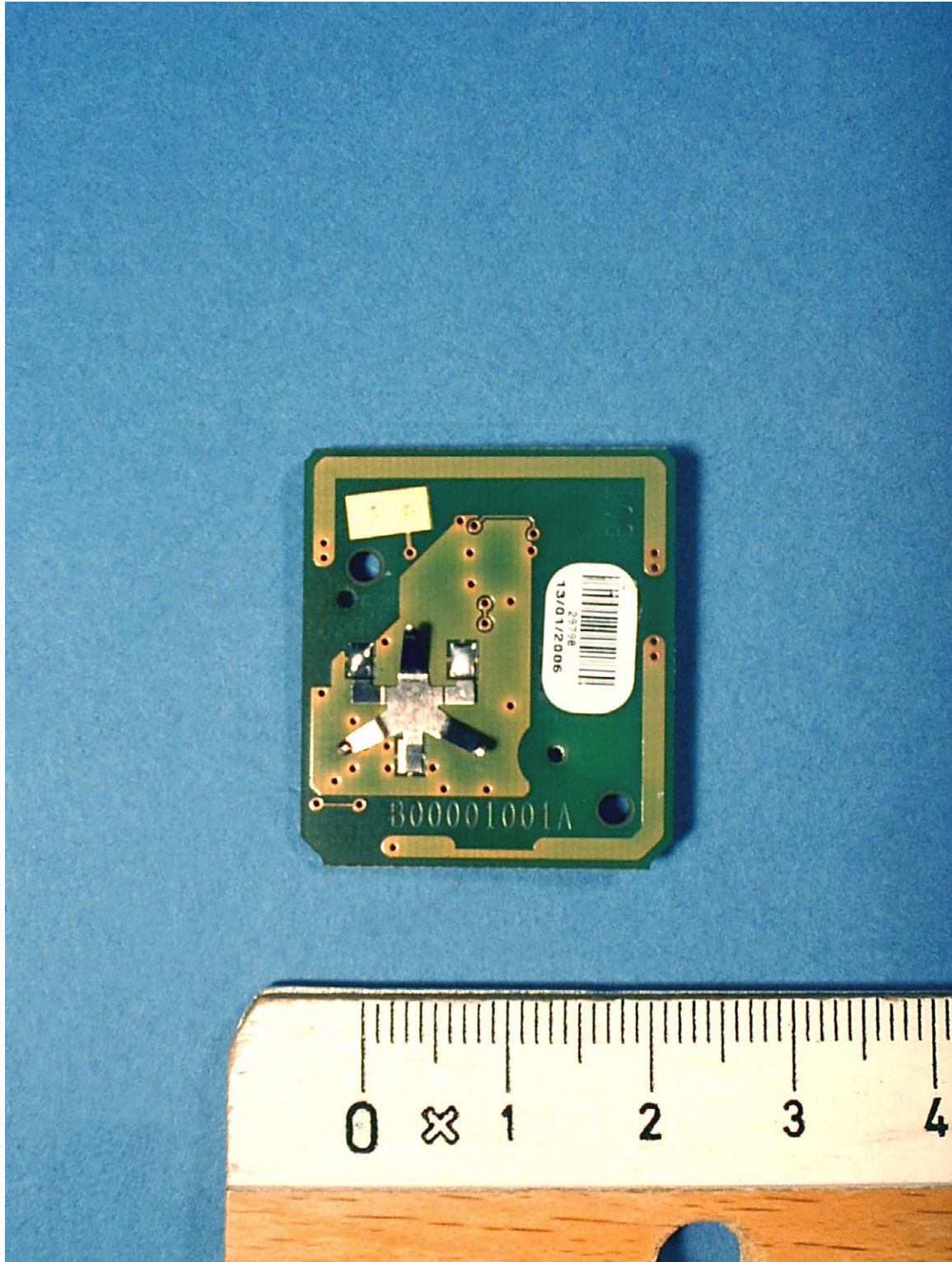
Photograph 2: Transmitter, PCB solder side
