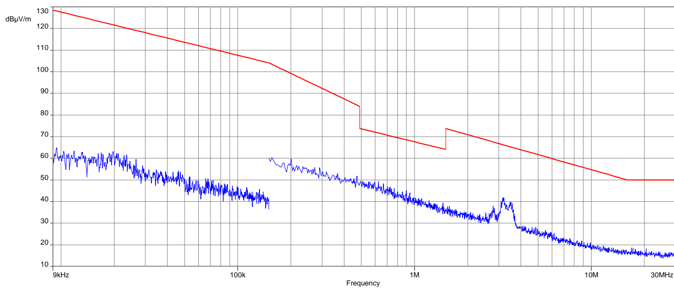
Plot 3: 9 kHz to 30 MHz, high channel, CW
