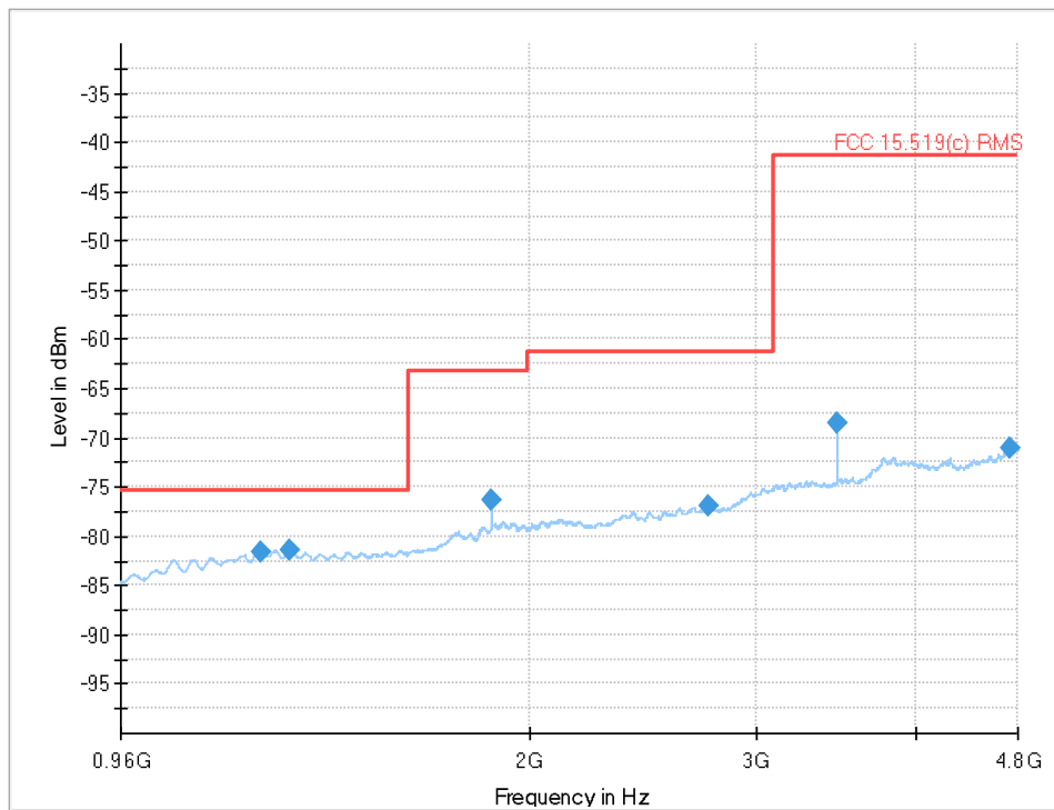
Plot 11: 960 MHz to 4.8 GHz (Limit acc. to §15.519 (c)), UWB test mode, DUT-B, CH5
