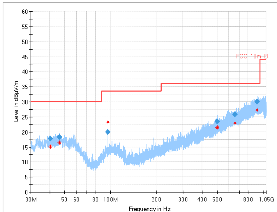
Plot 9: 30 MHz to 1 GHz, UWB test mode, DUT-B, CH5
