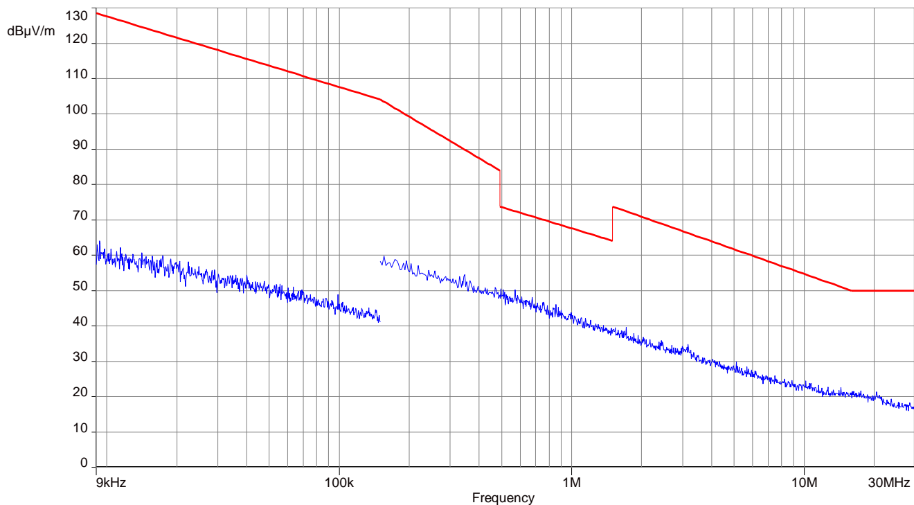
Plot 7: 9 kHz to 30 MHz, UWB test mode, DUT-B, CH5
