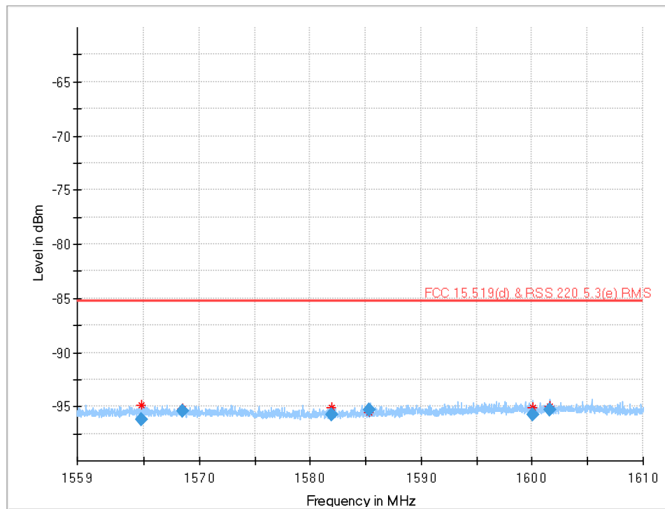
Plot 25: 1559 MHz to 1610 MHz (§15.519 (d)), UWB test mode, DUT-B, CH5
