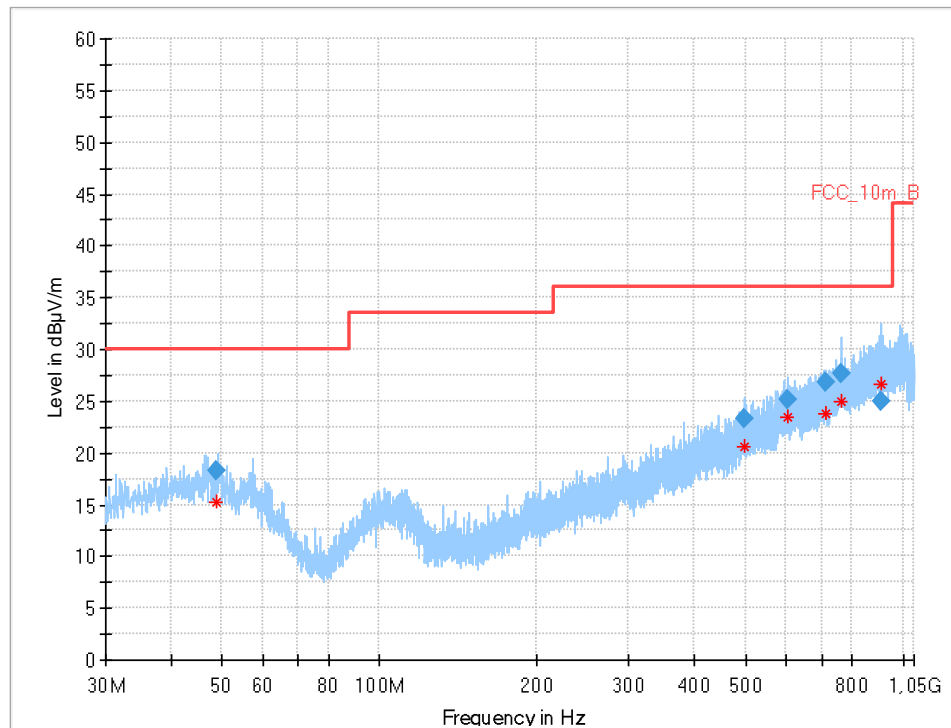
Plot 10: 30 MHz to 1 GHz, UWB test mode, DUT-B, CH9
