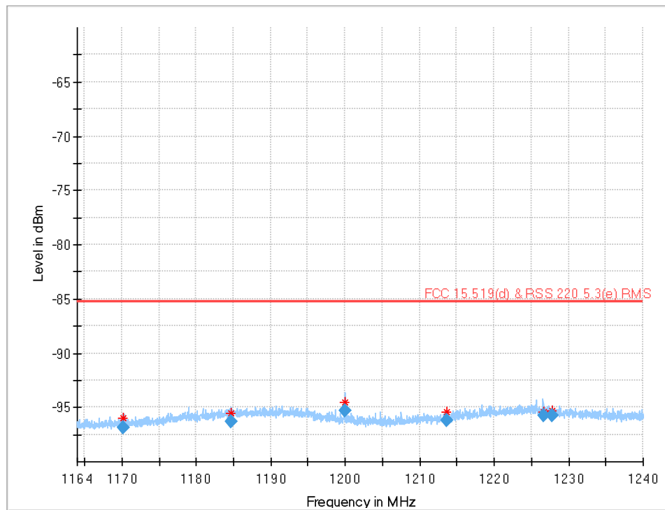
Plot 23: 1164 MHz to 1240 MHz (§15.519 (d)), UWB test mode, DUT-B, CH5
