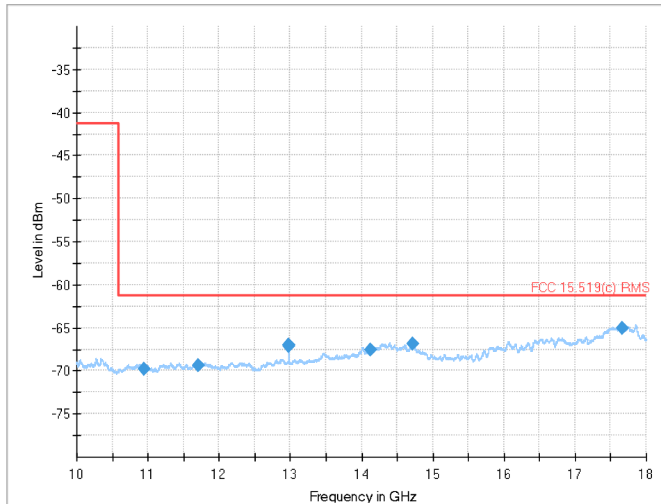
Plot 15: 10 GHz to 18 GHz, UWB test mode, DUT-B, CH5
