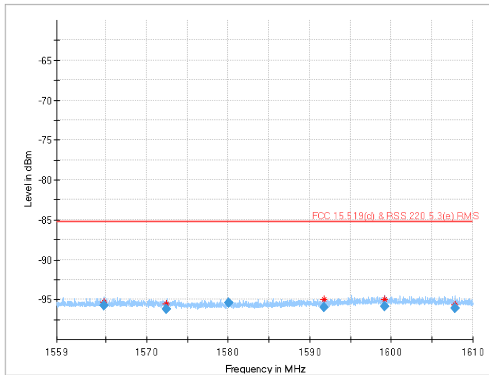
Plot 26: 1559 MHz to 1610 MHz (§15.519 (d)), UWB test mode, DUT-B, CH9
