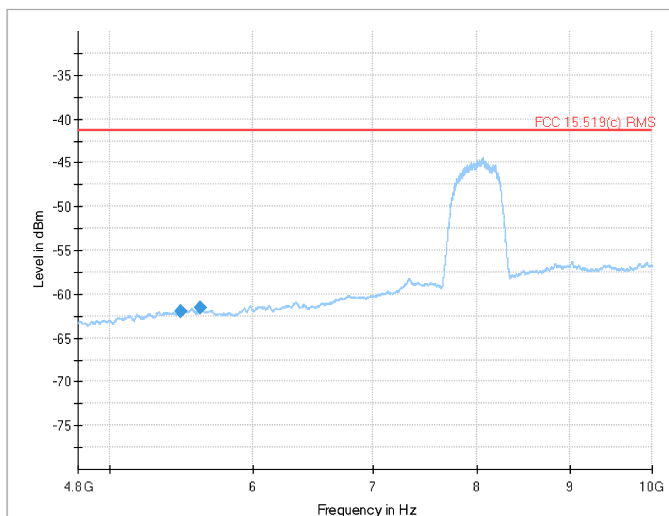
Plot 14: 4.8 GHz to 10 GHz, UWB test mode, DUT-B, CH9
