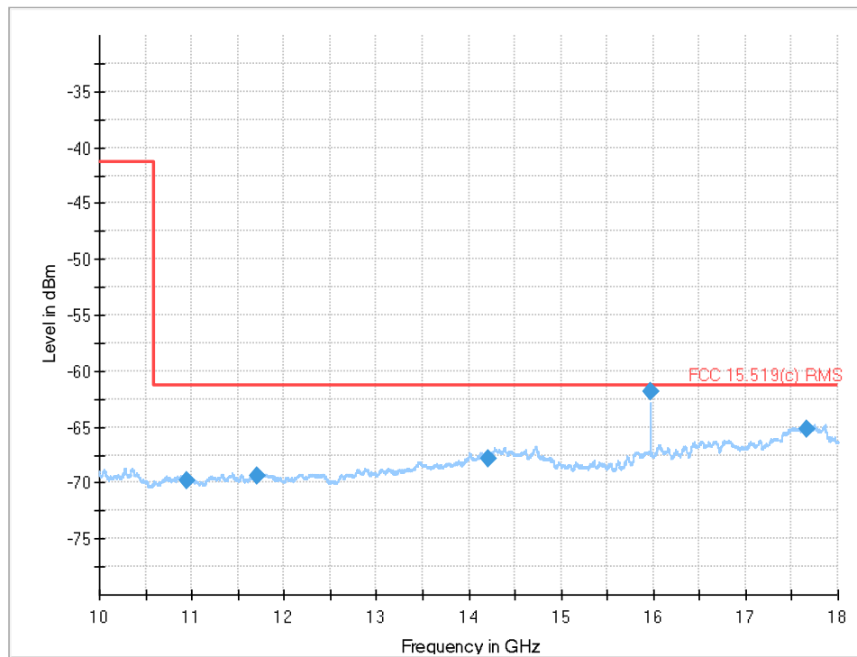
Plot 16: 10 GHz to 18 GHz, UWB test mode, DUT-B, CH9
