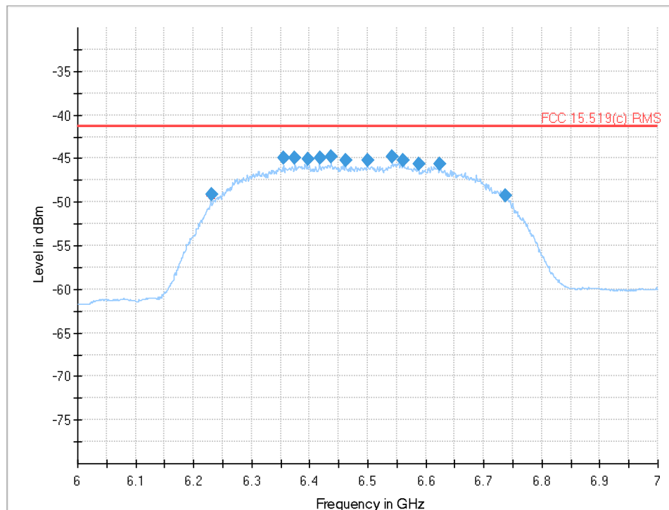
Plot 3: Fundamental emission (UWB test mode): RMS, DUT-B, CH5
