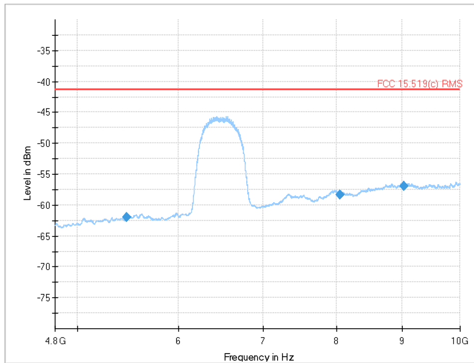
Plot 13: 4.8 GHz to 10 GHz, UWB test mode, DUT-B, CH5
