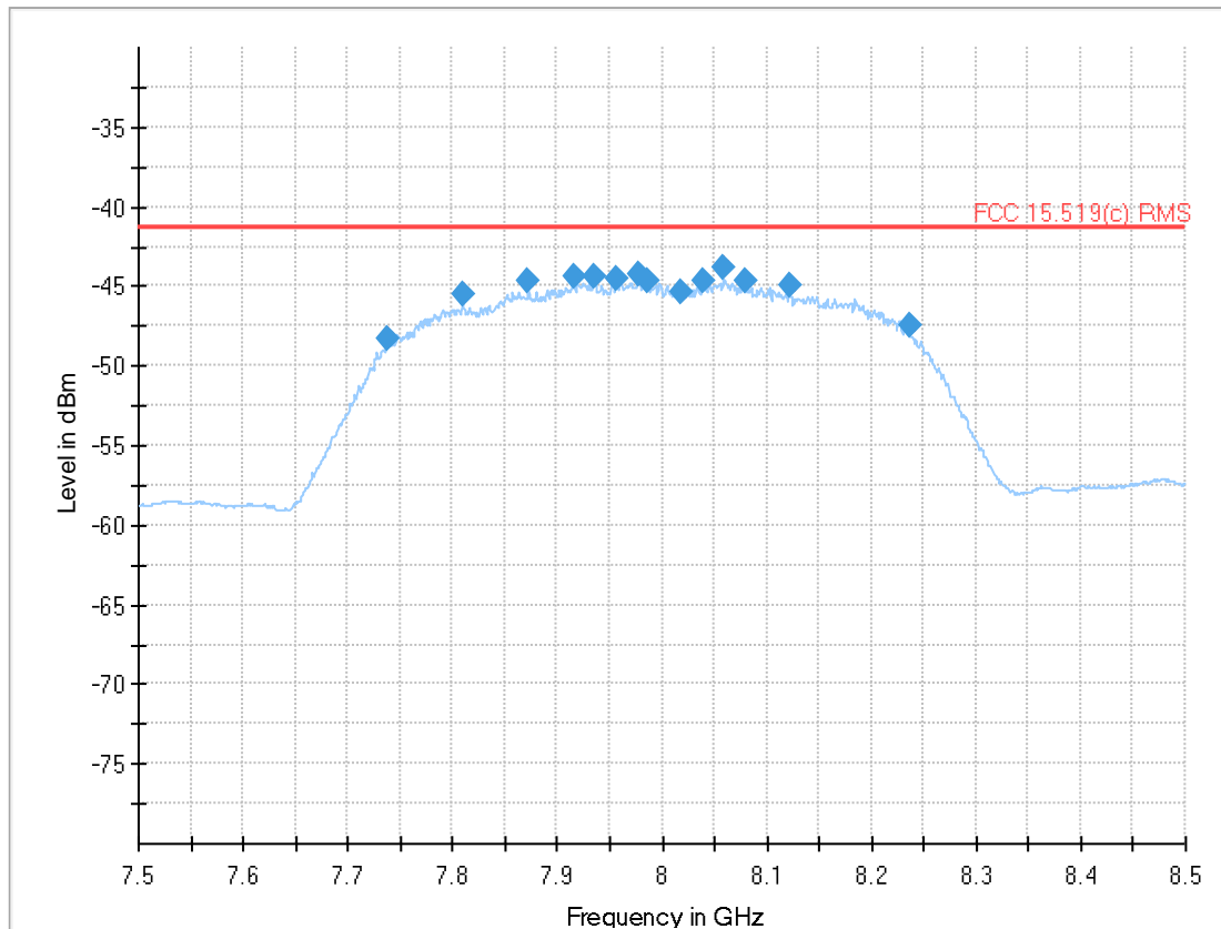
Plot 4: Fundamental emission (UWB test mode): RMS, DUT-B, CH9
