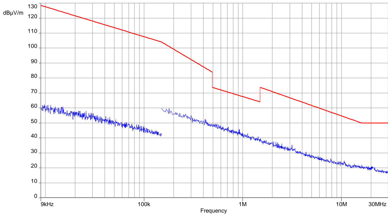
Plot 8: 9 kHz to 30 MHz, UWB test mode, DUT-B, CH9
