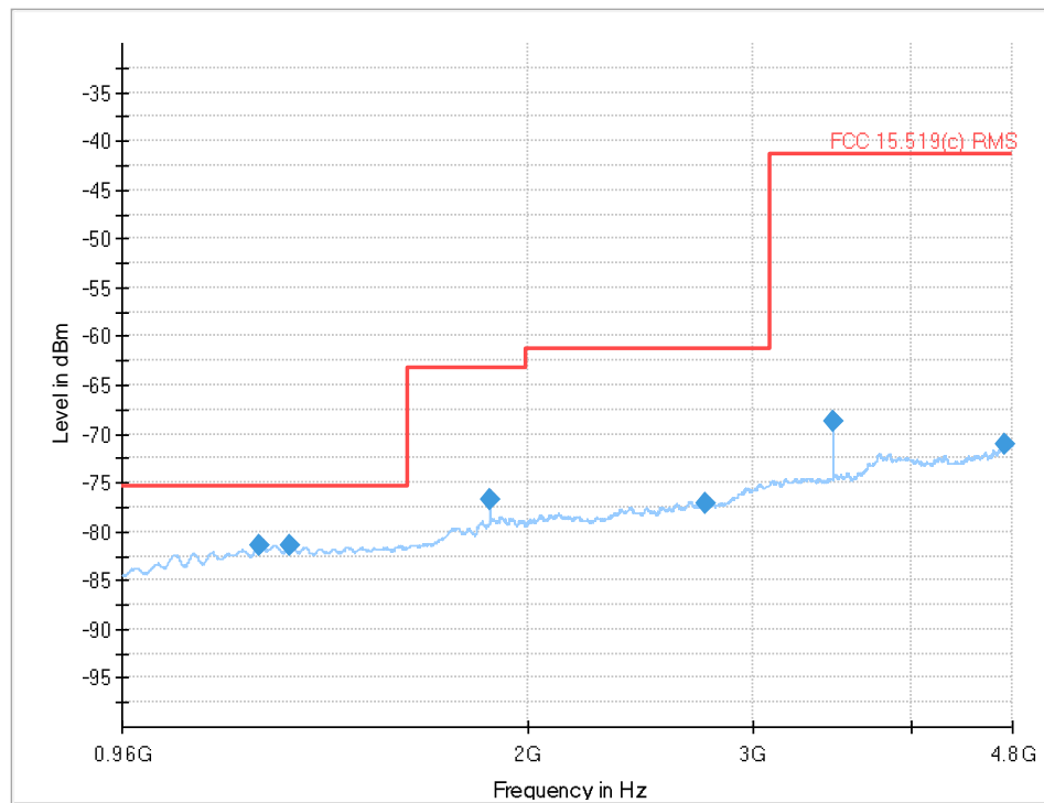
Plot 12: 960 MHz to 4.8 GHz (Limit acc. to §15.519 (c)), UWB test mode, DUT-B, CH9
