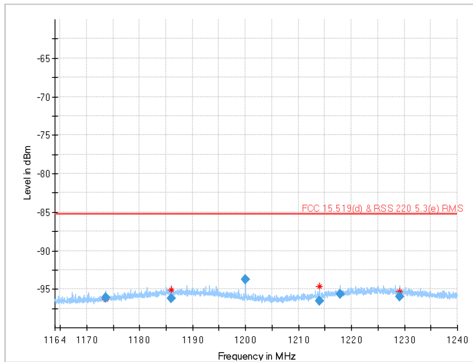
Plot 24: 1164 MHz to 1240 MHz (§15.519 (d)), UWB test mode, DUT-B, CH9
