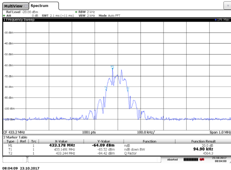
Plot 2: 20 dB bandwidth, 433.20 MHz
