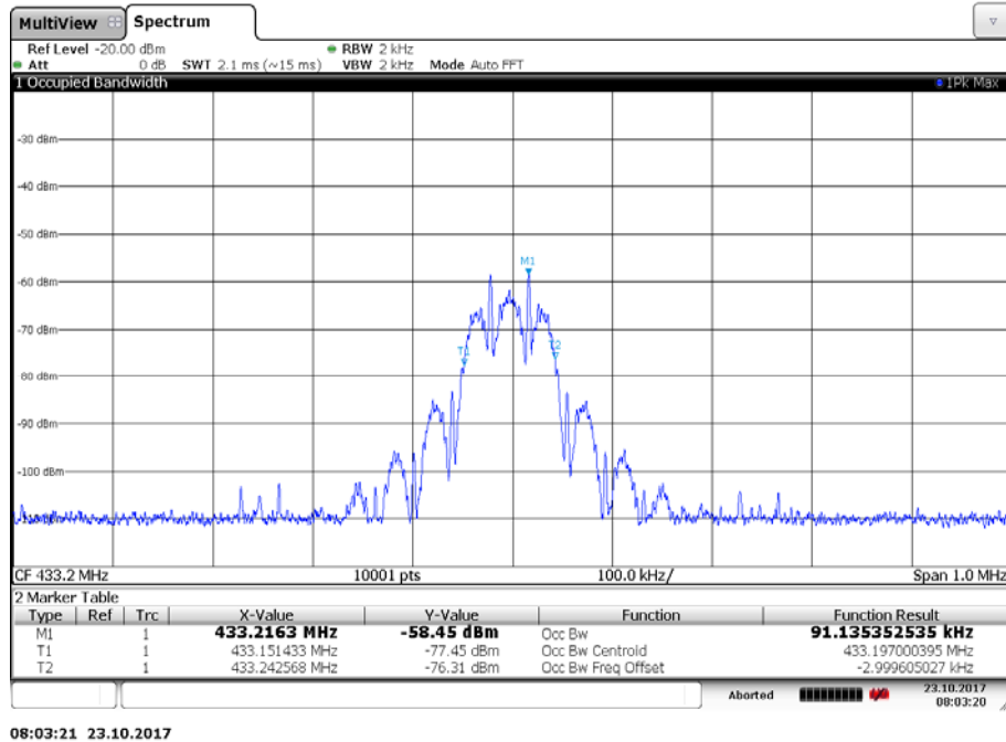
Plot 1: 99% bandwidth, 433.20 MHz
