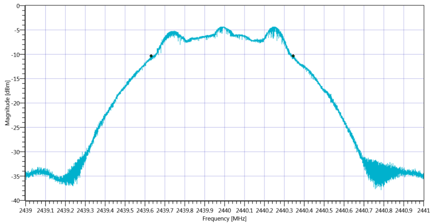
Plot_FCC Part 15.247 Bandwidth 6dB DTS ~ BT LE 1 Msps_02122019_182108.png
