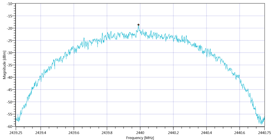
Plot_FCC Part 15.247 Peak Power Spectral Density DTS ~ BT LE 1 Msp_02122019_182247.png
