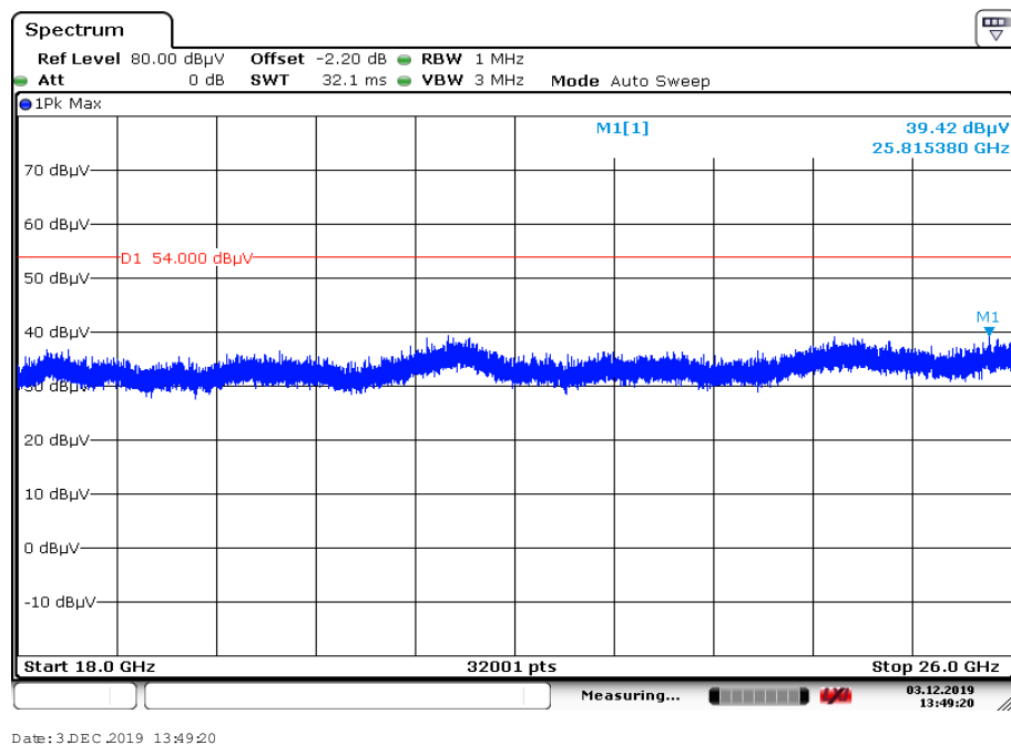
Plot 4: 18 GHz to 26 GHz, TX mode, 2440 MHz, vertical & horizontal polarization, 1 Msps, antenna 1
