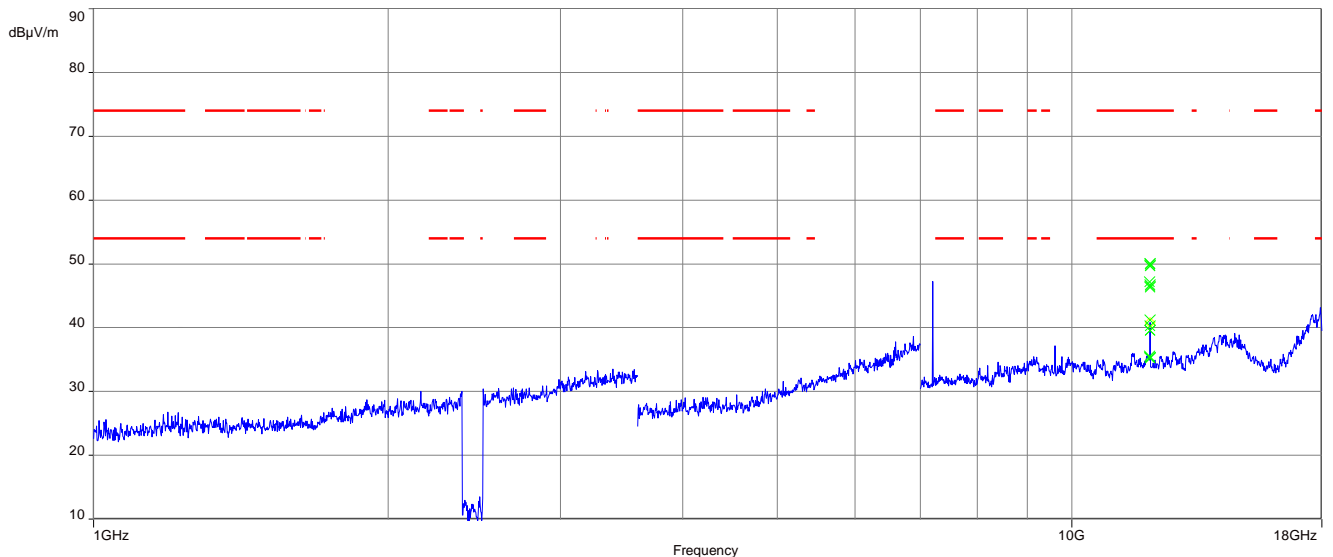
Plot 7: 1 GHz to 18 GHz, TX mode, 2402 MHz, vertical & horizontal polarization, 1 Msps, antenna 2
