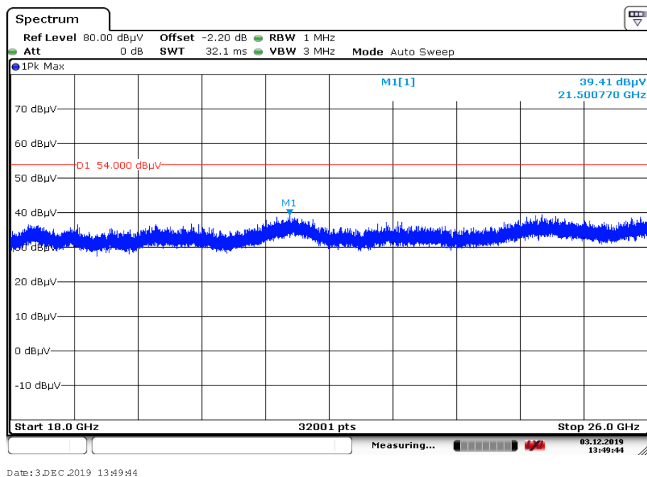
Plot 10: 18 GHz to 26 GHz, TX mode, 2440 MHz, vertical & horizontal polarization, 1 Msps, antenna 2
