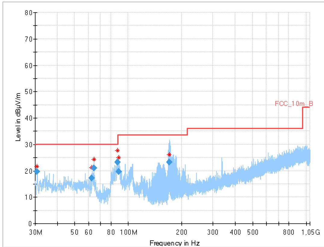
Plot 4: 30 MHz to 1 GHz, TX mode, 2402 MHz, vertical & horizontal polarization, 1 Msps, antenna 2
