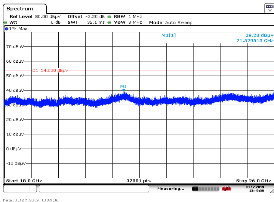
Plot 8: 18 GHz to 26 GHz, TX mode, 2402 MHz, vertical & horizontal polarization, 1 Msps, antenna 2
