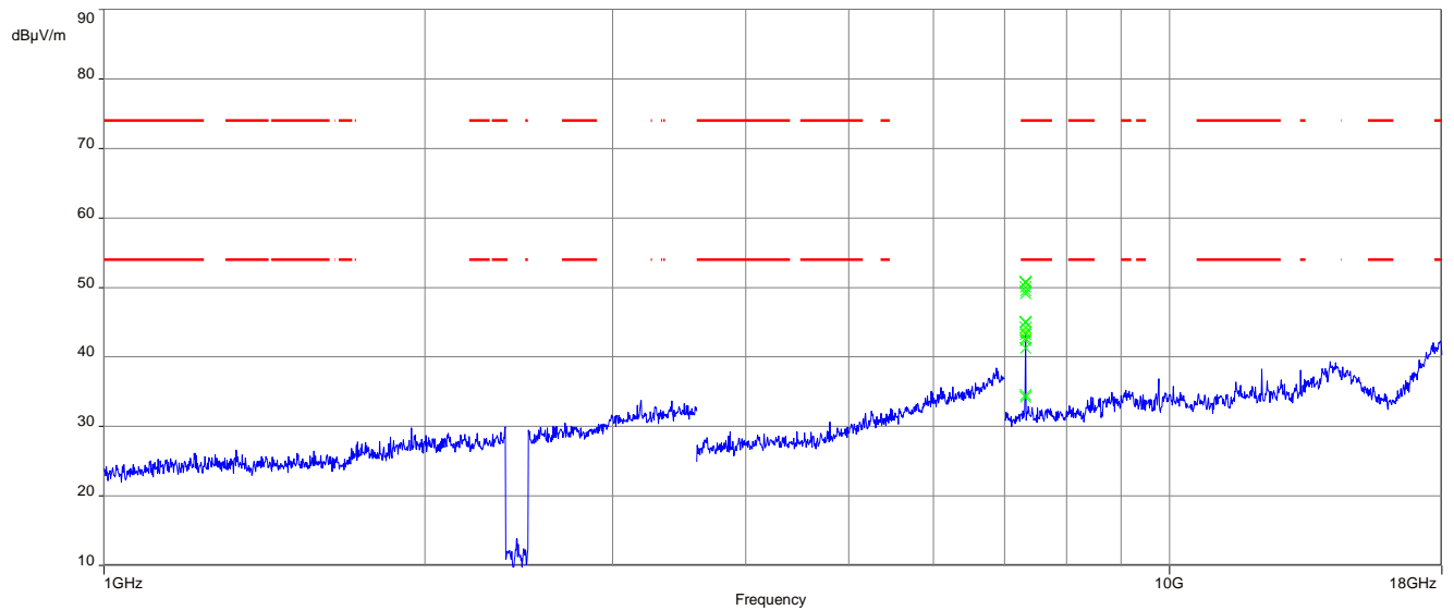
Plot 9: 1 GHz to 18 GHz, TX mode, 2440 MHz, vertical & horizontal polarization, 1 Msps, antenna 2
