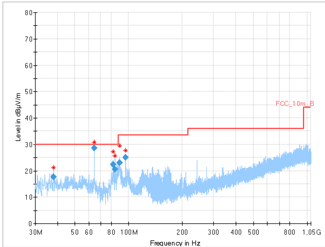
Plot 2: 30 MHz to 1 GHz, TX mode, 2440 MHz, vertical & horizontal polarization, 1 Msps, antenna 1
