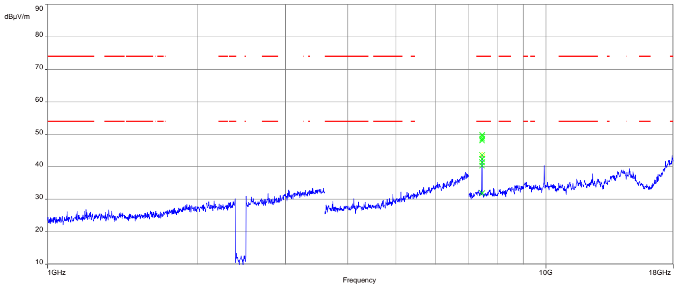
Plot 5: 1 GHz to 18 GHz, TX mode, 2480 MHz, vertical & horizontal polarization, 1 Msps, antenna 1
