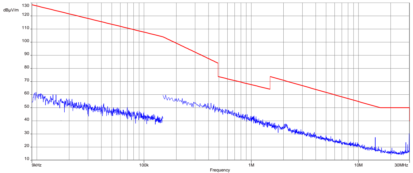
Plot 6: 9 kHz to 30 MHz, 2480 MHz, transmit mode, 1 Msps, antenna 2
