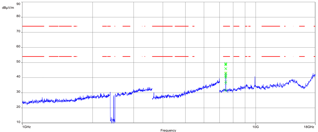
Plot 11: 1 GHz to 18 GHz, TX mode, 2480 MHz, vertical & horizontal polarization, 1 Msps, antenna 2
