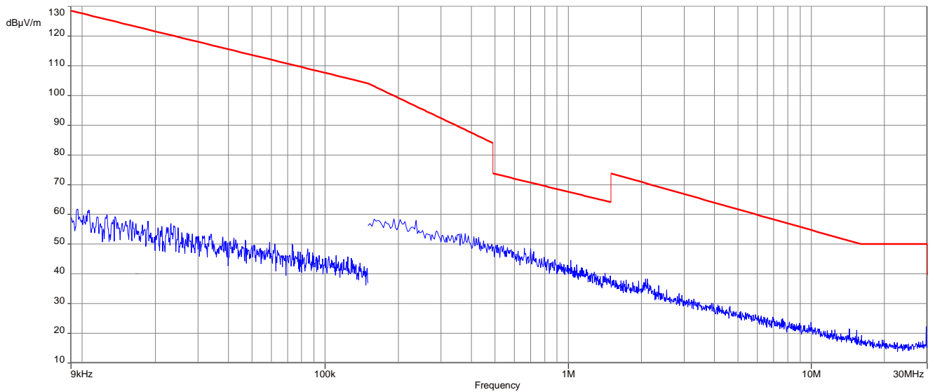
Plot 4: 9 kHz to 30 MHz, 2402 MHz, transmit mode, 1 Msps, antenna 2
