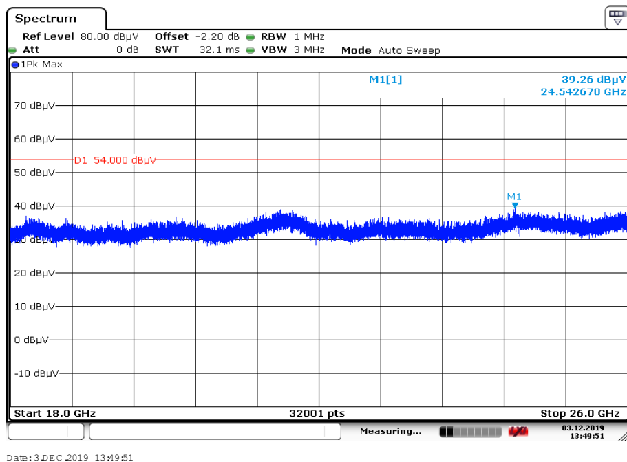
Plot 12: 18 GHz to 26 GHz, TX mode, 2480 MHz, vertical & horizontal polarization, 1 Msps, antenna 2
