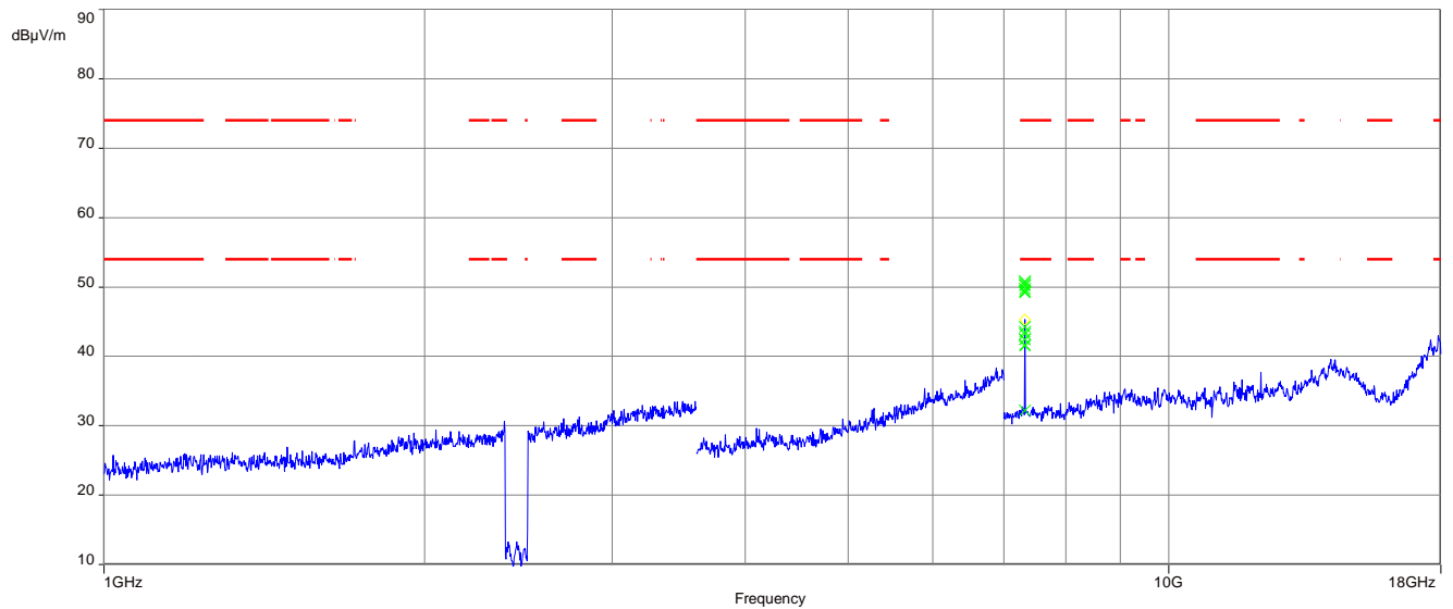
Plot 3: 1 GHz to 18 GHz, TX mode, 2440 MHz, vertical & horizontal polarization, 1 Msps, antenna 1
