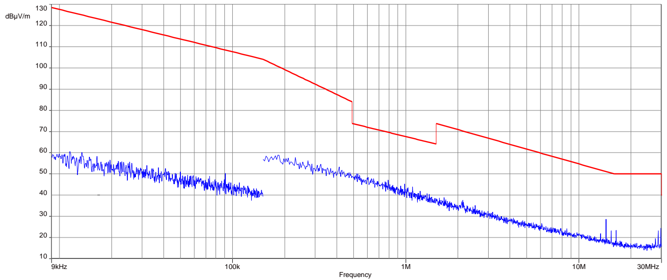
Plot 5: 9 kHz to 30 MHz, 2440 MHz, transmit mode, 1 Msps, antenna 2
