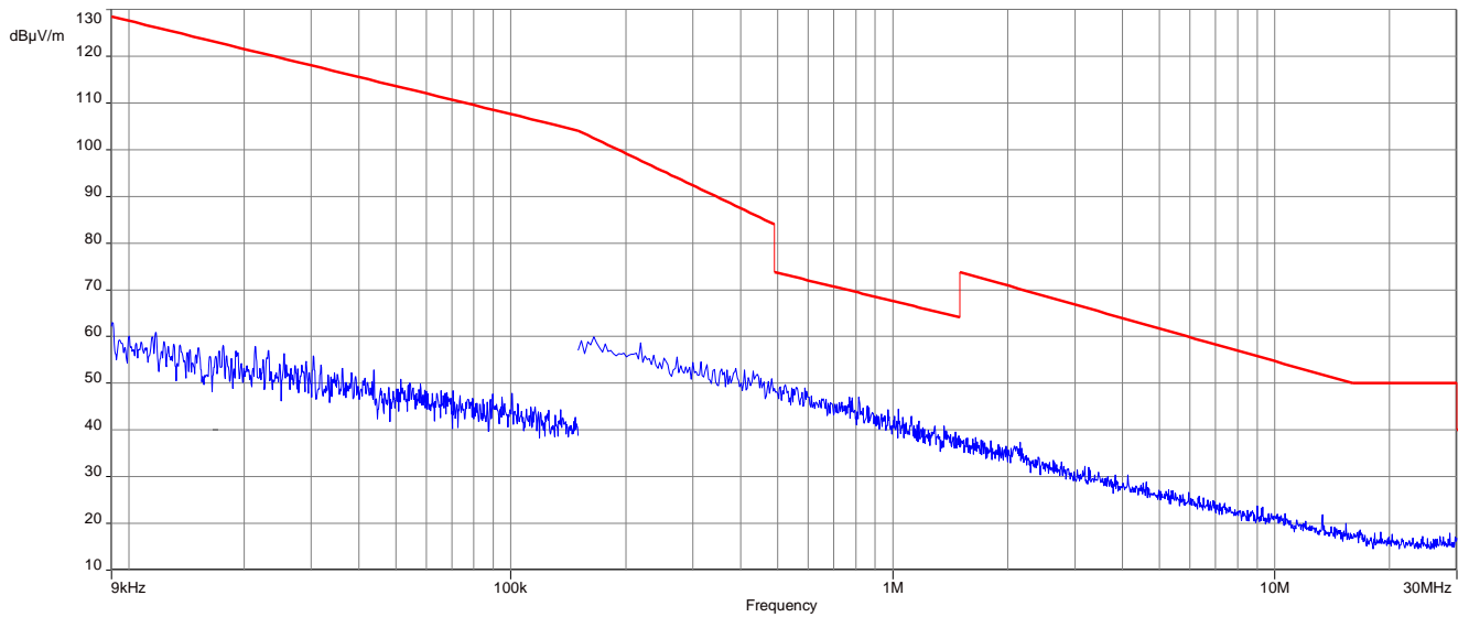
Plot 3: 9 kHz to 30 MHz, 2480 MHz, transmit mode, 1 Msps, antenna 1
