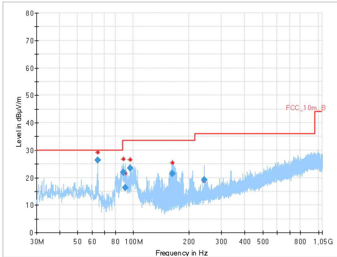
Plot 3: 30 MHz to 1 GHz, TX mode, 2480 MHz, vertical & horizontal polarization, 1 Msps, antenna 1
