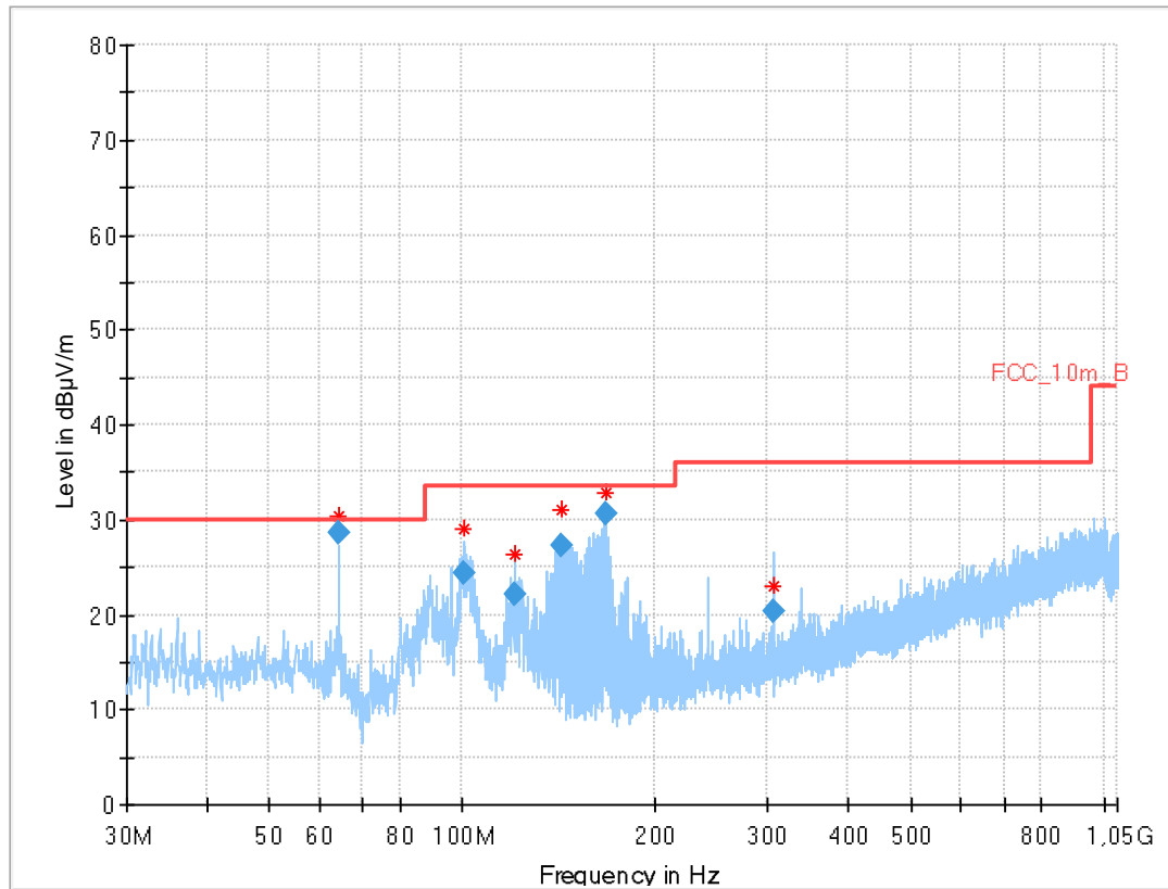
Plot 6: 30 MHz to 1 GHz, TX mode, 2480 MHz, vertical & horizontal polarization, 1 Msps, antenna 2
