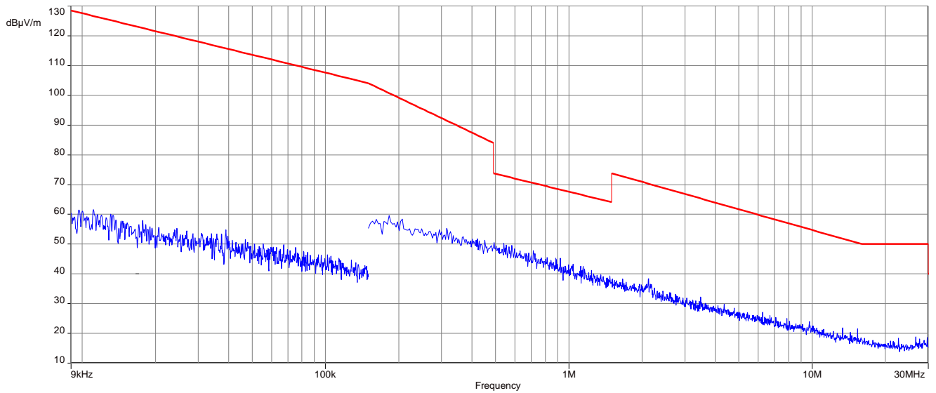
Plot 1: 9 kHz to 30 MHz, 2402 MHz, transmit mode, 1 Msps, antenna 1
