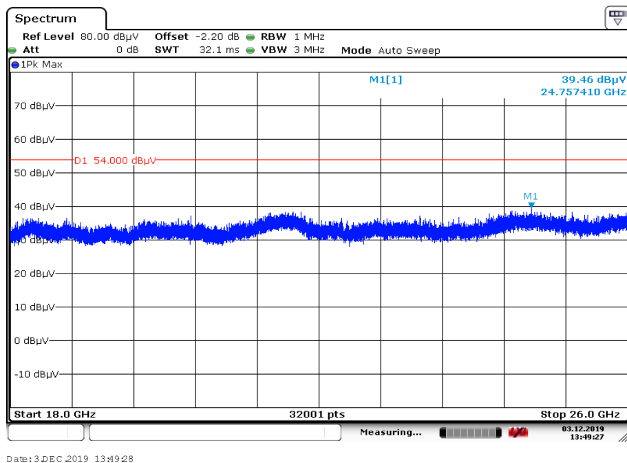
Plot 6: 18 GHz to 26 GHz, TX mode, 2480 MHz, vertical & horizontal polarization, 1 Msps, antenna 1
