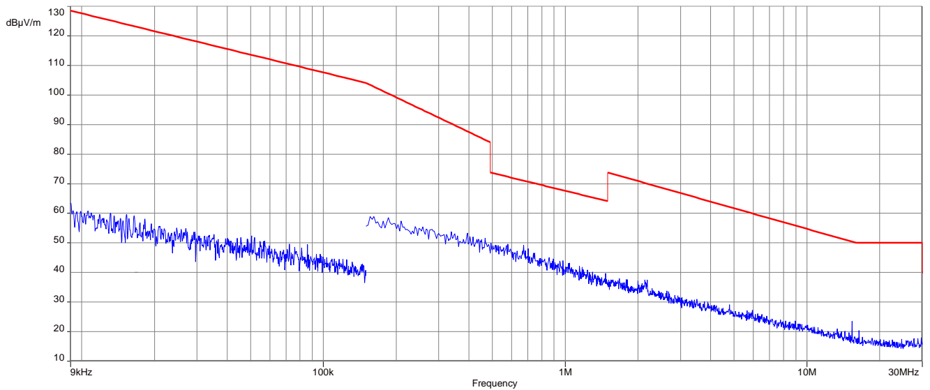
Plot 2: 9 kHz to 30 MHz, 2440 MHz, transmit mode, 1 Msps, antenna 1
