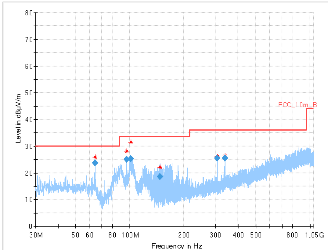
Plot 5: 30 MHz to 1 GHz, TX mode, 2440 MHz, vertical & horizontal polarization, 1 Msps, antenna 2
