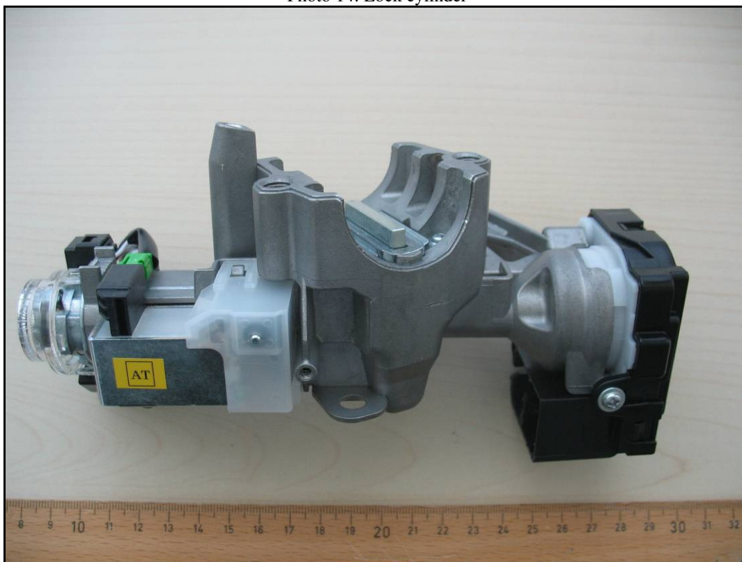
Photo 14: Lock cylinder
