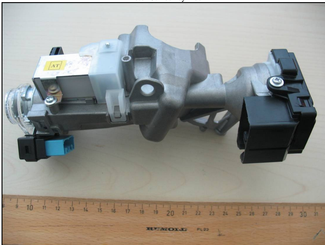
Photo 16: Lock cylinder
