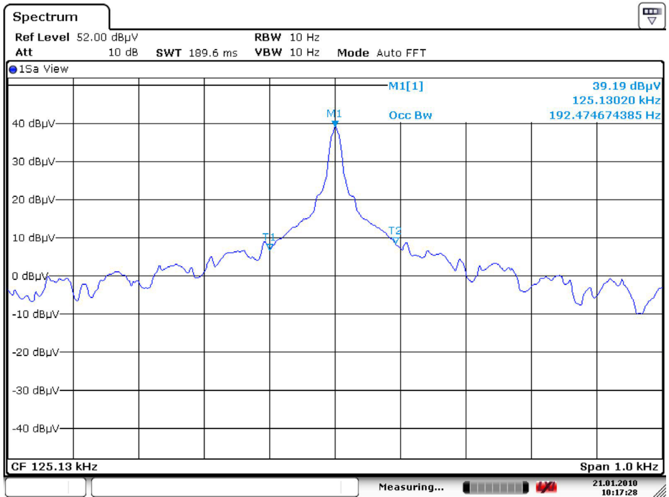
Plot 1: Occupied bandwidth of the emission, 192.5 Hz as measured with a spectrum analyzer
