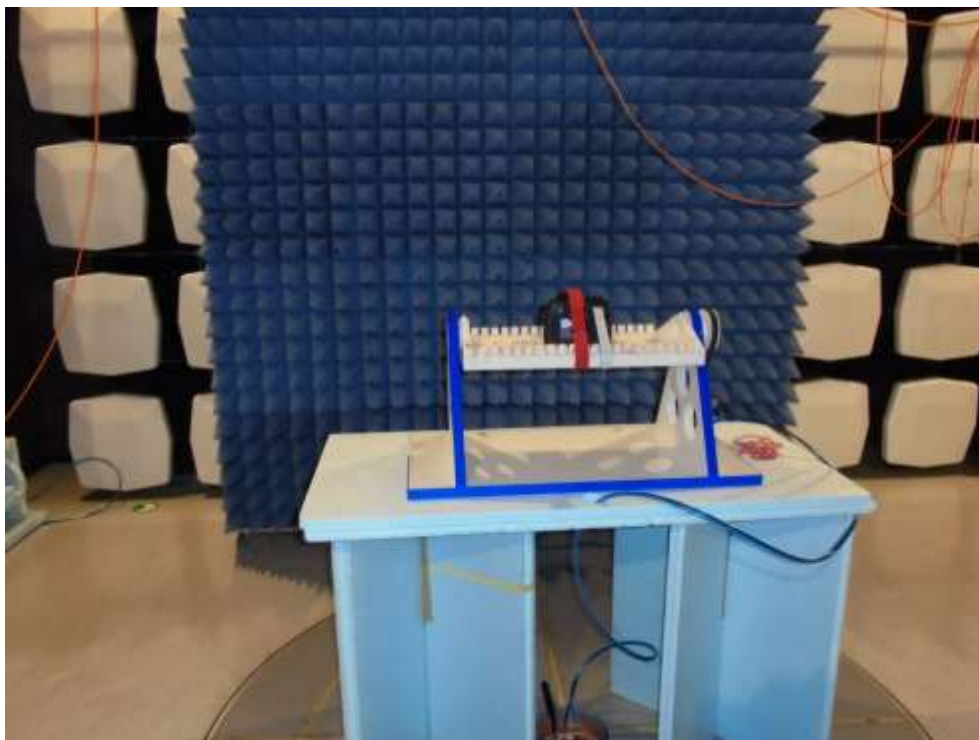
Radiated field strength measurements ( f < 1\text{GHz} )
