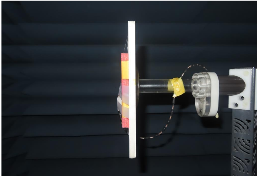
Fig. 6-1 Test position FS Front View
