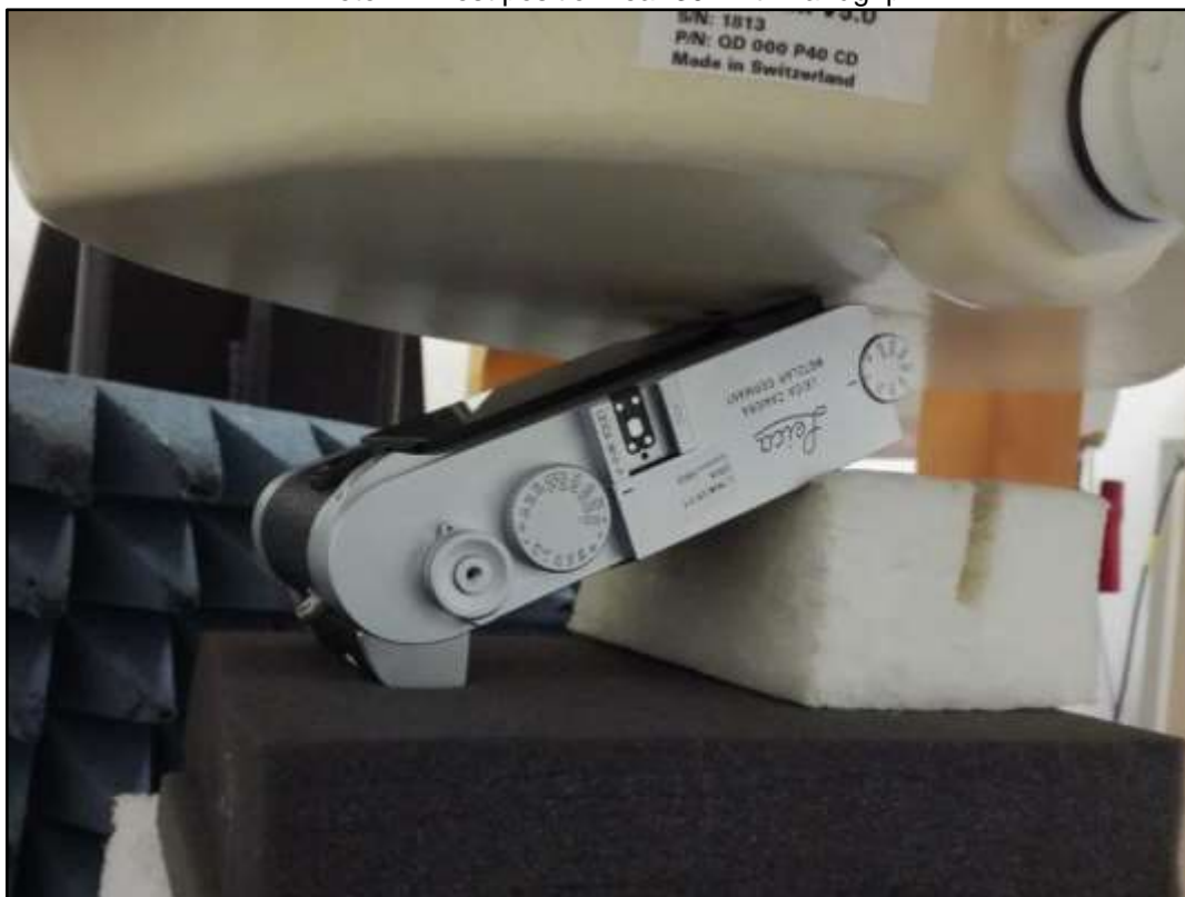
Photo 12: Test position rear 30° with handgrip
