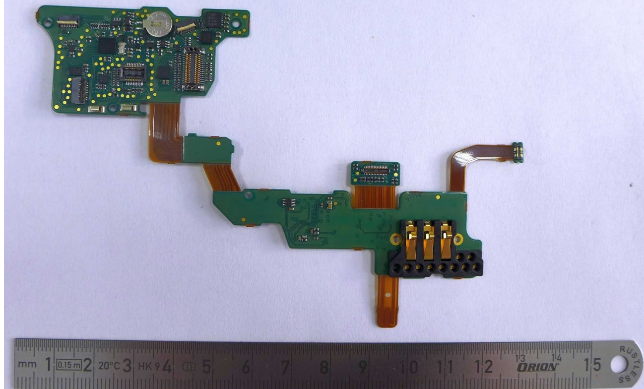
H Mainboard
