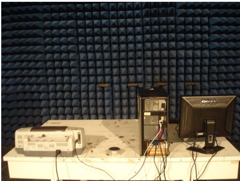
Photo of Setup for Radiated Emission (Charging Mode)
