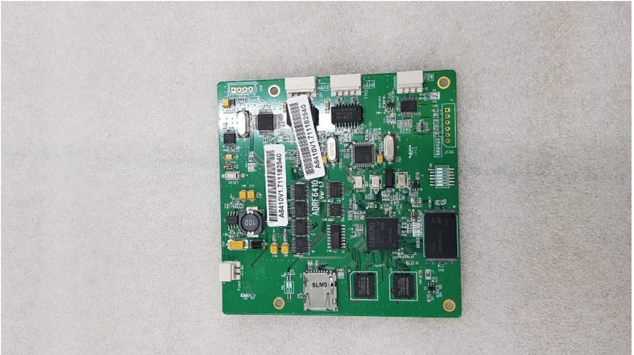
CPU Board TOP
