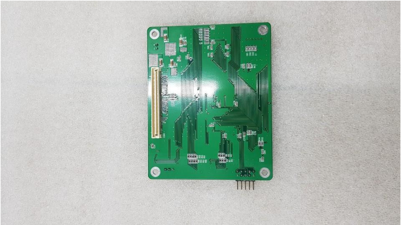
DSP CTRL Board BOTTOM
