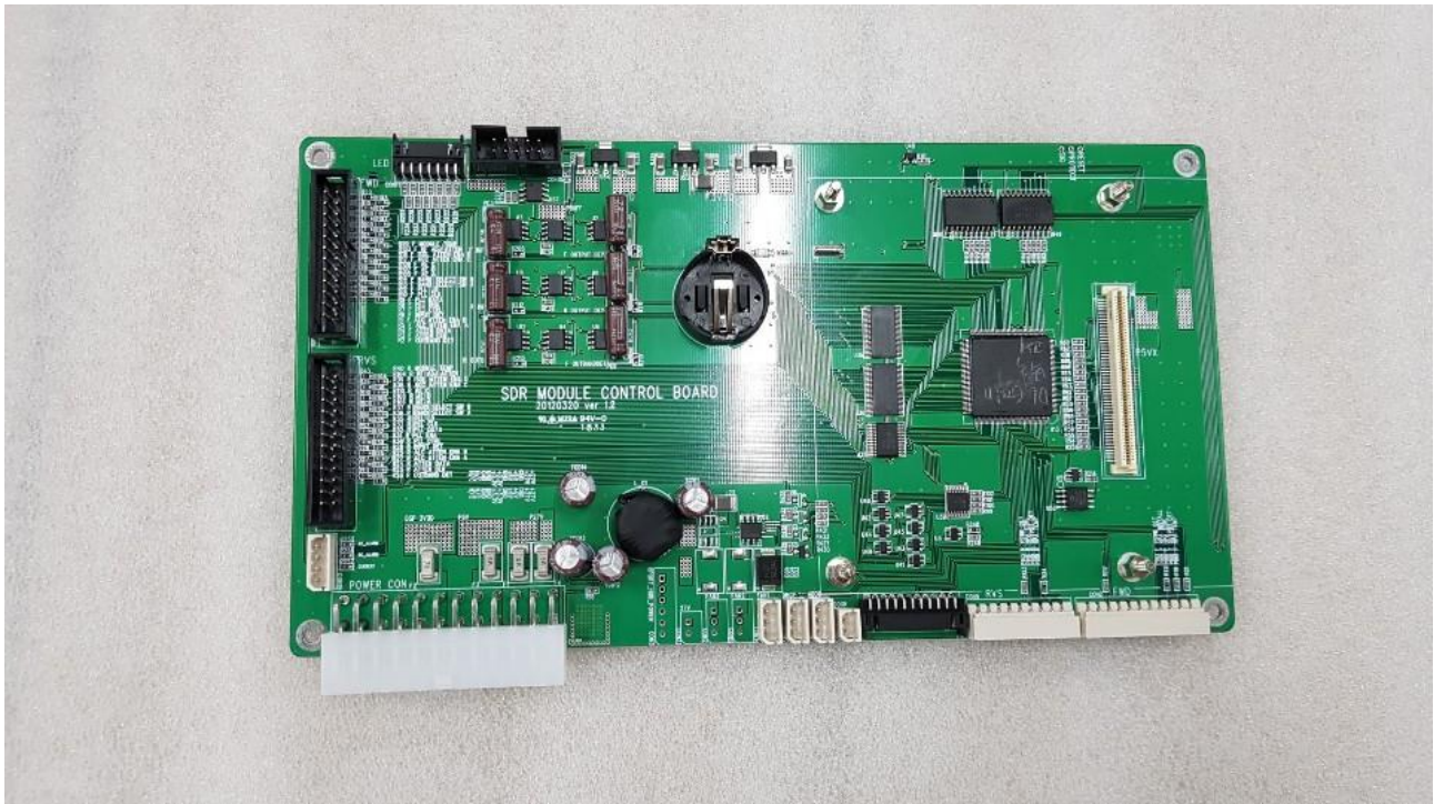
[SDR-CHANNEL BASE B'd TOP]
