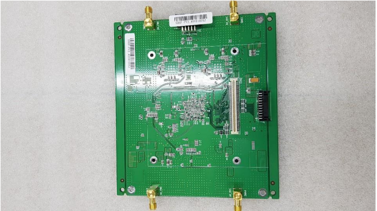
[SDR-DSP B'd BOTTOM]
