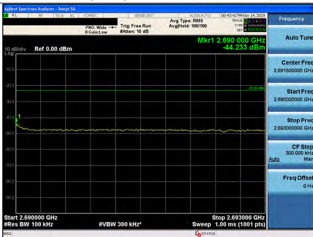
Out-of-band (single test signals) / BRS/EBS / Uplink / 5G NR 100M / Upper
