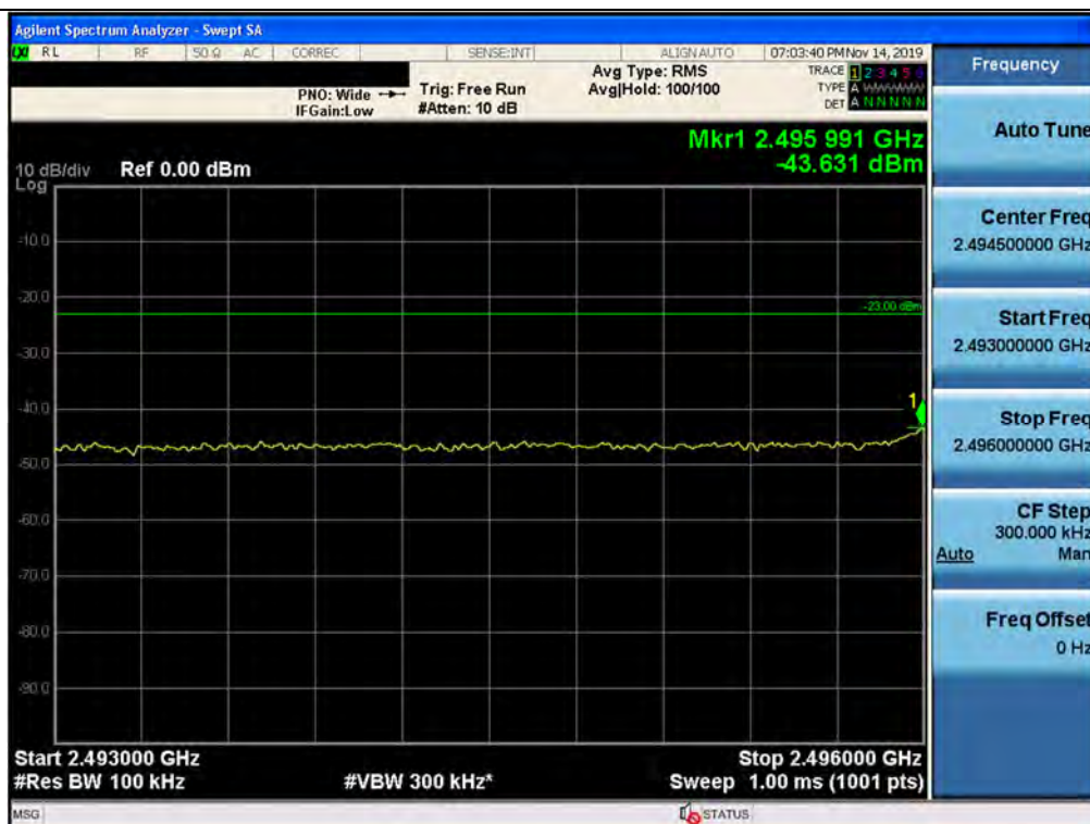
Out-of-band (single test signals) / BRS/EBS / Uplink / 5G NR 100M / Lower
