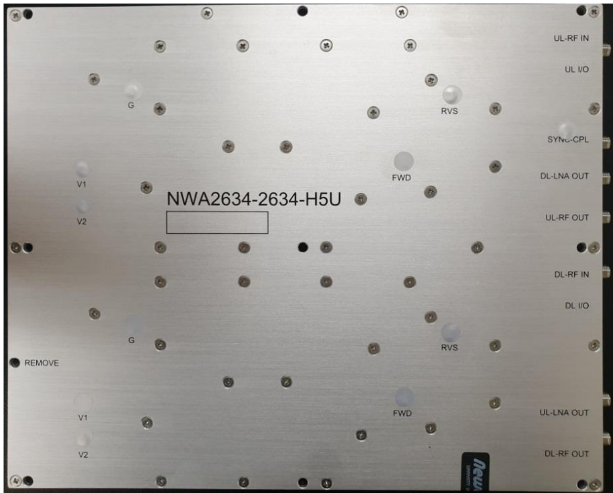
[HPA_1]
