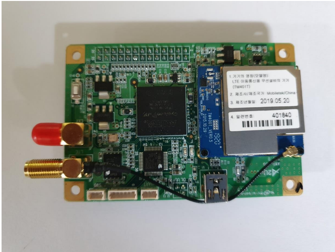
[Control Board_4]
