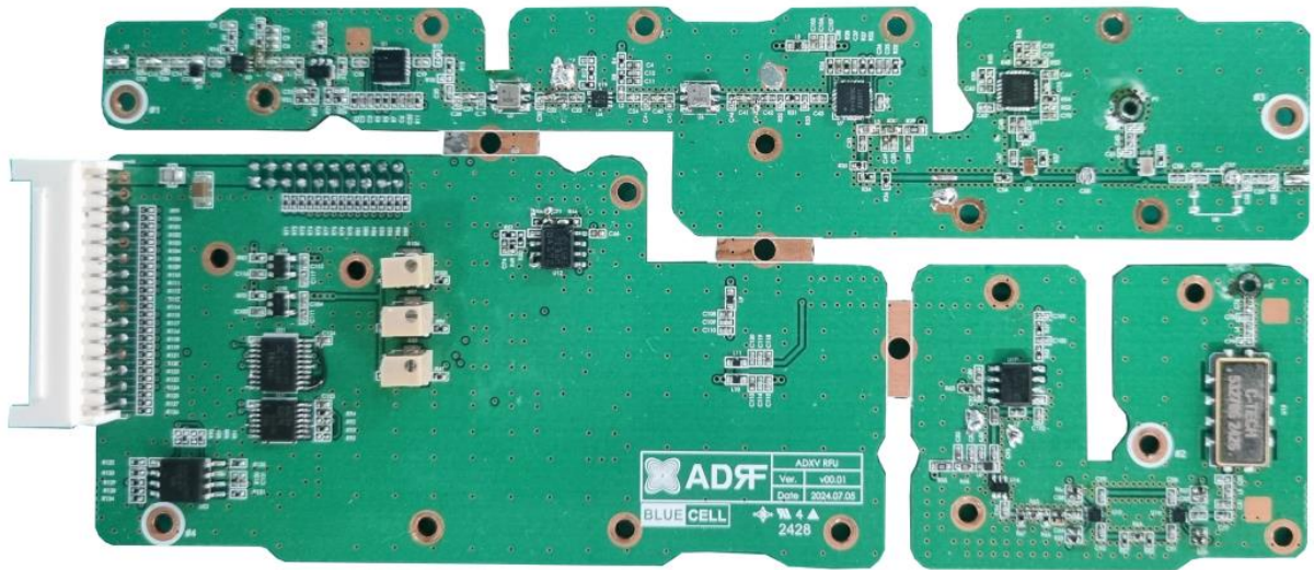
RFU Top Board
