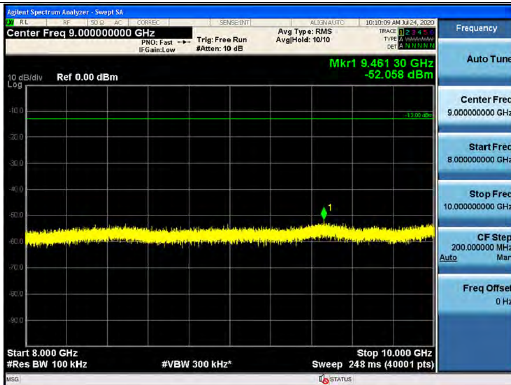
Spurious / 928 ~ 929 MHz / Downlink / P25 Phase 1 / Middle / 8 GHz ~ 10 GHz
