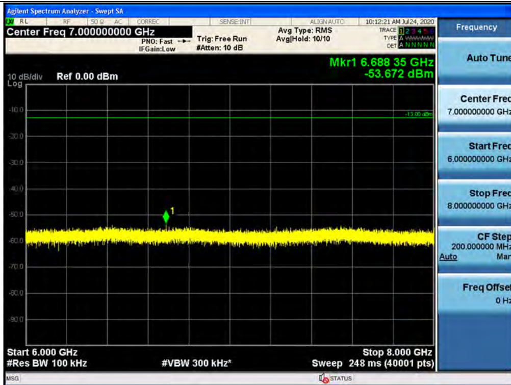
Spurious / 928 ~ 929 MHz / Downlink / P25 Phase 1 / High / 6 GHz ~ 8 GHz
