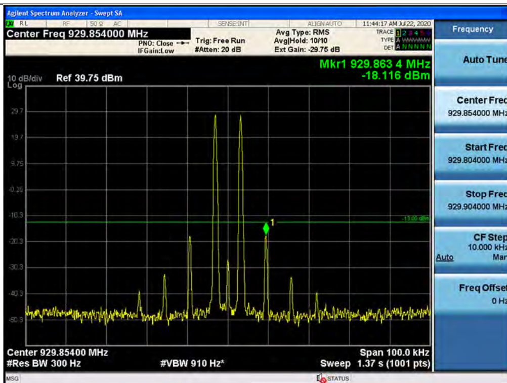
+3 dB above Out-of-band (two adjacent test signals) / 929 ~ 930 MHz / Downlink / CW
