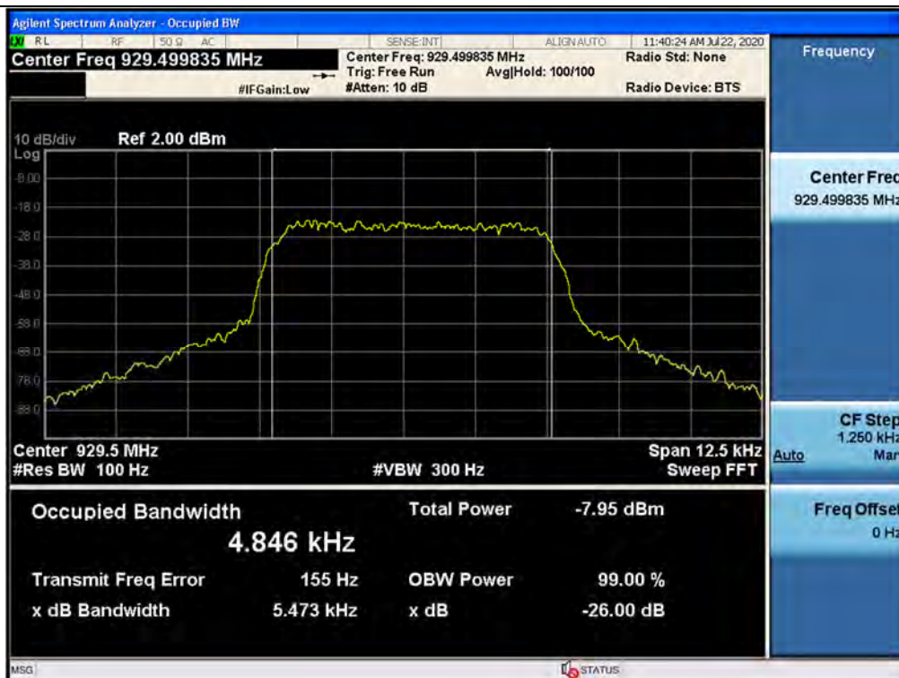
Input / 929 ~ 930 MHz / Downlink / P25 Phase 2
