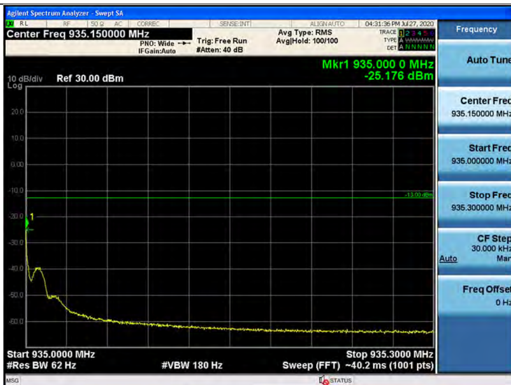
Out-of-band (two adjacent test signals) / 932 ~ 935 MHz / Downlink / P25 Phase 2 / Upper
