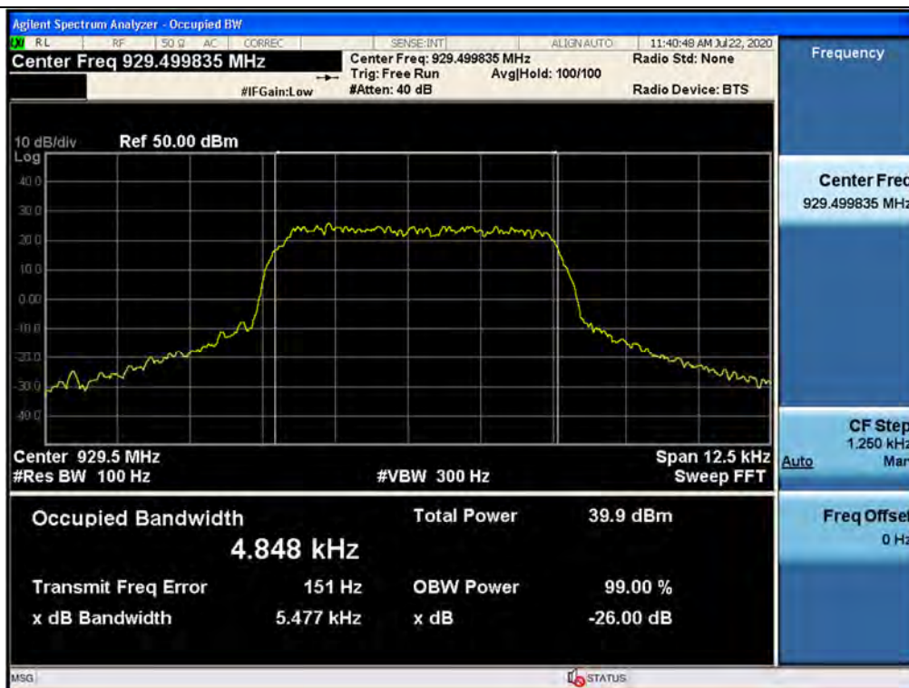
Output / 929 ~ 930 MHz / Downlink / P25 Phase 2
