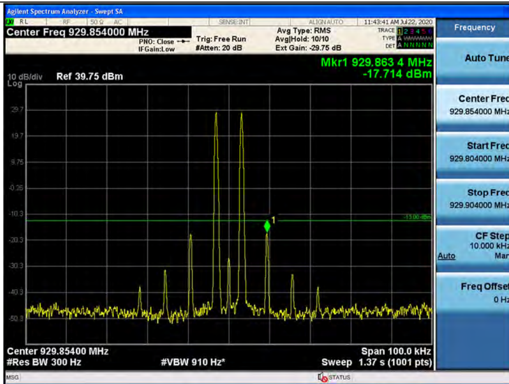
Out-of-band (two adjacent test signals) / 929 ~ 930 MHz / Downlink / CW
