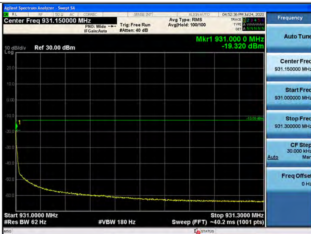
Out-of-band (single test signals) / 930 ~ 931 MHz / Downlink / P25 Phase 2 / Upper
