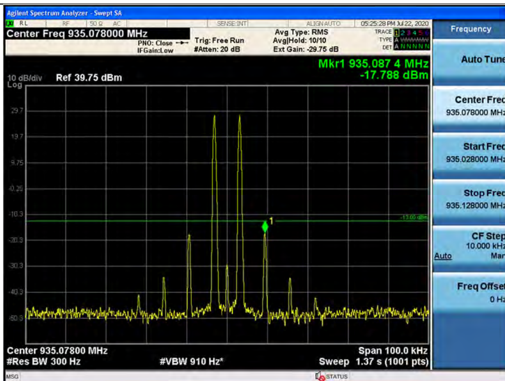
+3 dB above Out-of-band (two adjacent test signals) / 935 ~ 940 MHz / Downlink / CW
