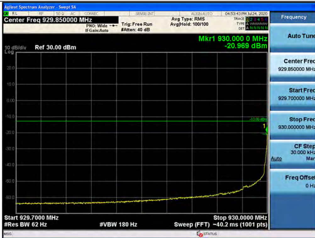
Out-of-band (single test signals) / 930 ~ 931 MHz / Downlink / P25 Phase 2 / Lower
