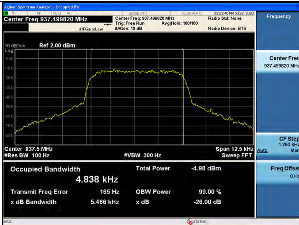
3 dB above the AGC threshold Input / 935 ~ 940 MHz / Downlink / P25 Phase 2
