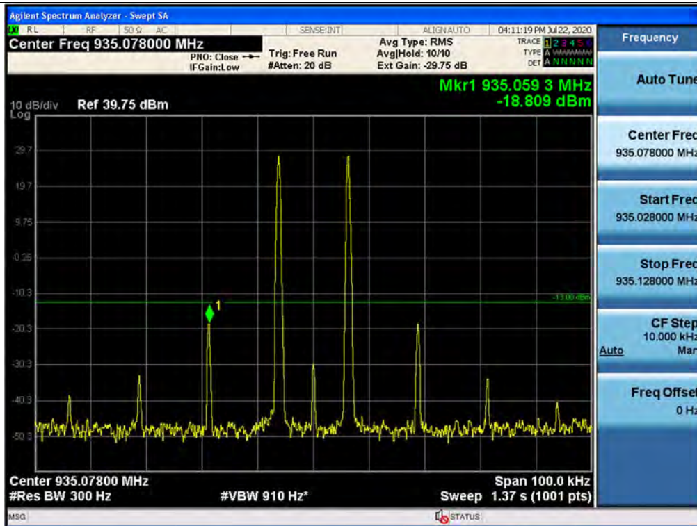
Out-of-band (two adjacent test signals) / 935 ~ 940 MHz / Downlink / CW
