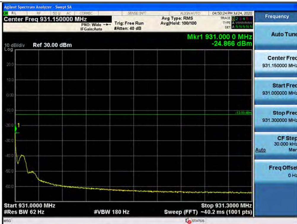
Out-of-band (two adjacent test signals) / 930 ~ 931 MHz / Downlink / P25 Phase 2 / Upper
