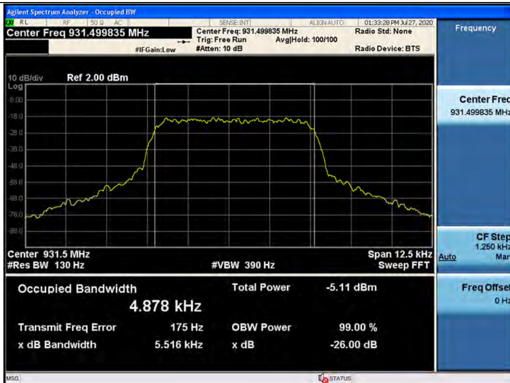
3 dB above the AGC threshold Input / 931 ~ 932 MHz / Downlink / P25 Phase 2
