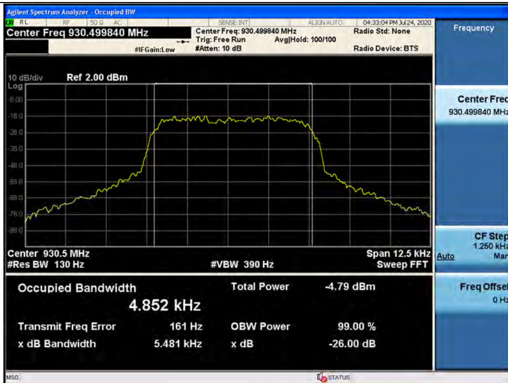
3 dB above the AGC threshold Input / 930 ~ 931 MHz / Downlink / P25 Phase 2
