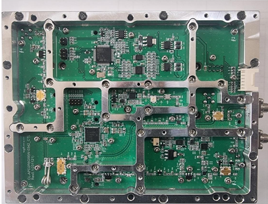
CTL PCB Internal
