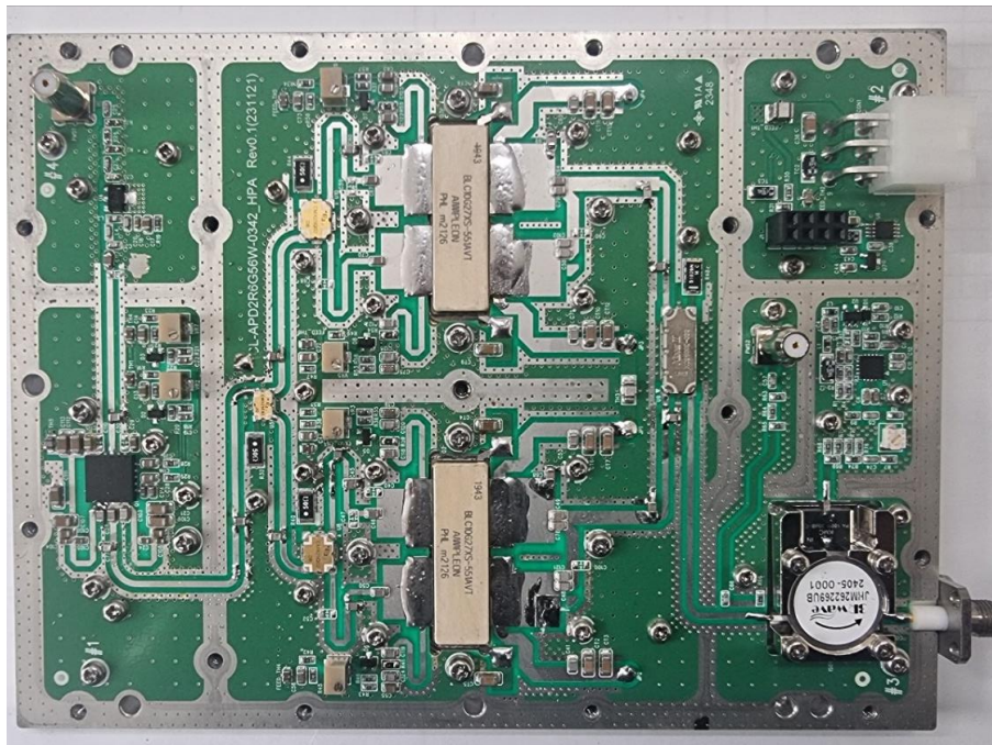
HPA PCB Internal
