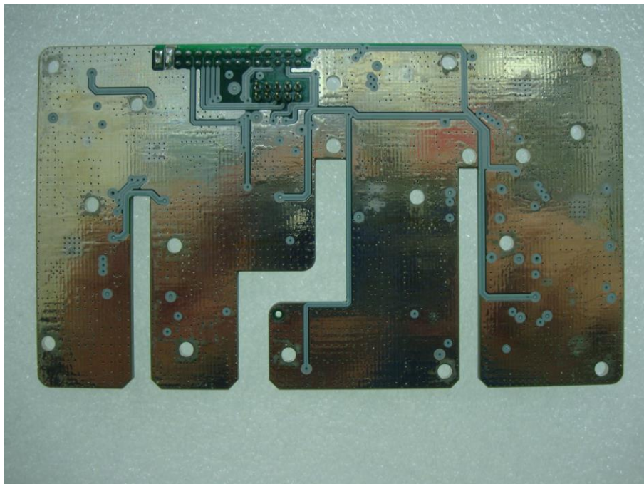
RF PBA BOTTOM
