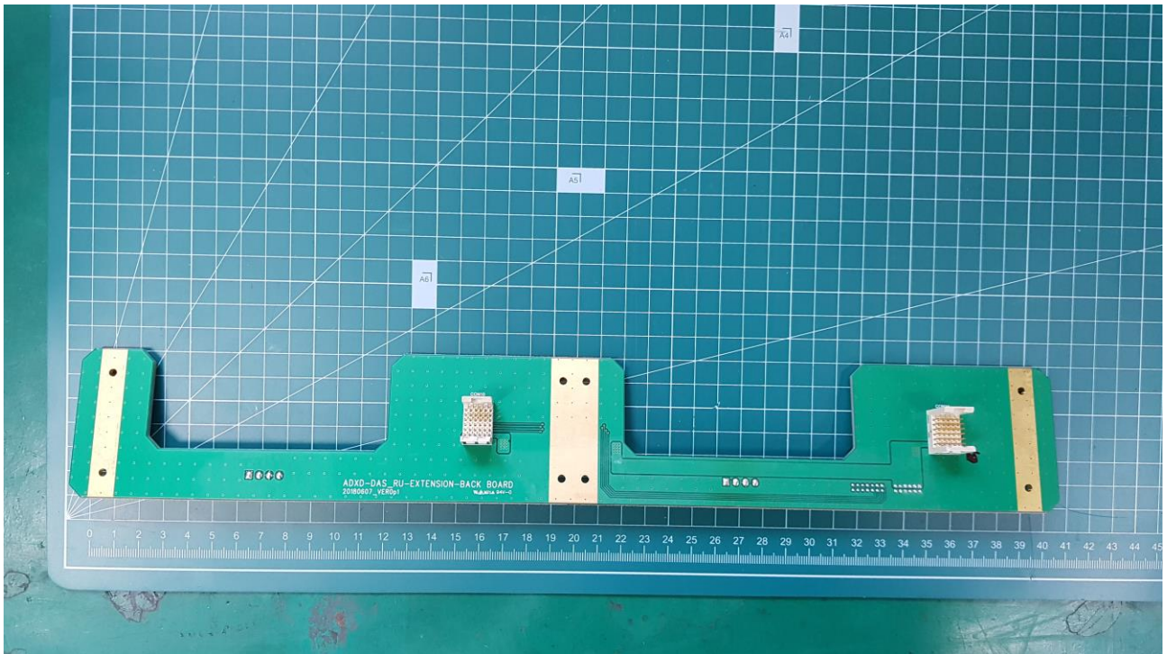
[R-Extension Back B'd TOP]
