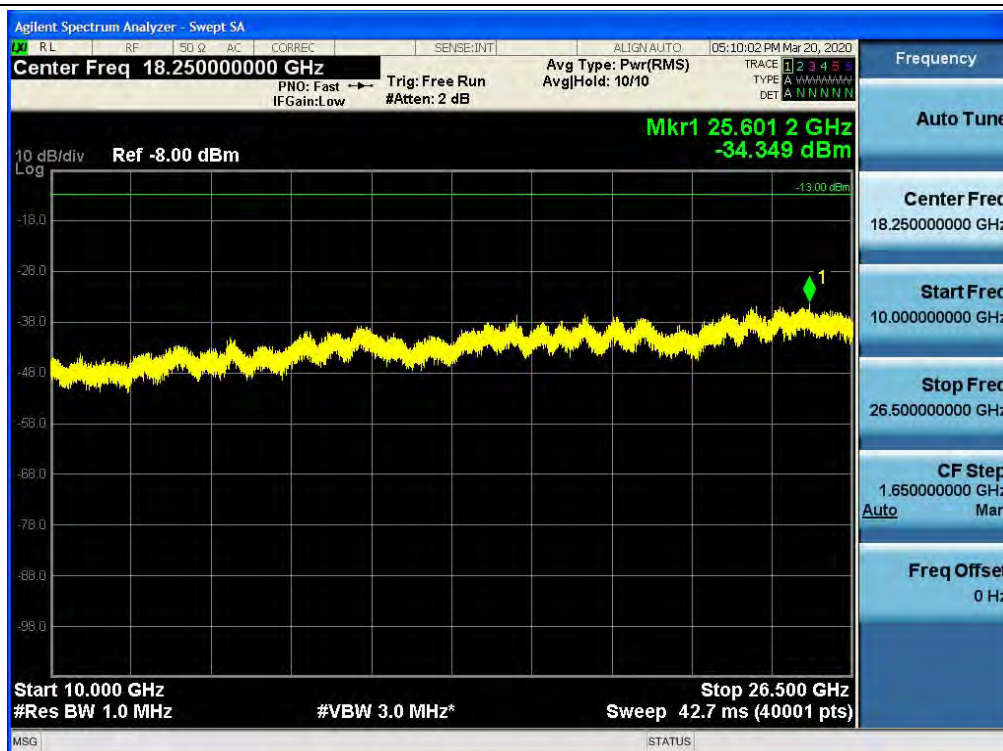
Spurious / BRS/EBS / Downlink / 5G NR 80M / Middle / 10 GHz ~ 26.5 GHz
