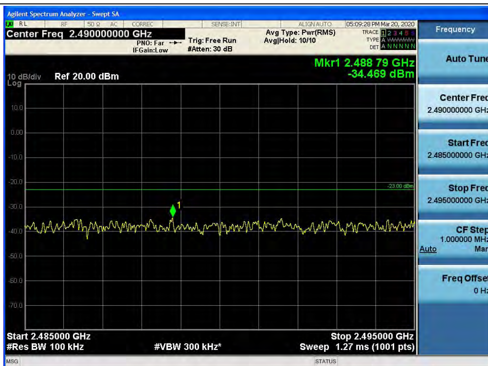
Spurious / BRS/EBS / Downlink / 5G NR 80M / Middle / Low Edge-10 ~ Low Edge
