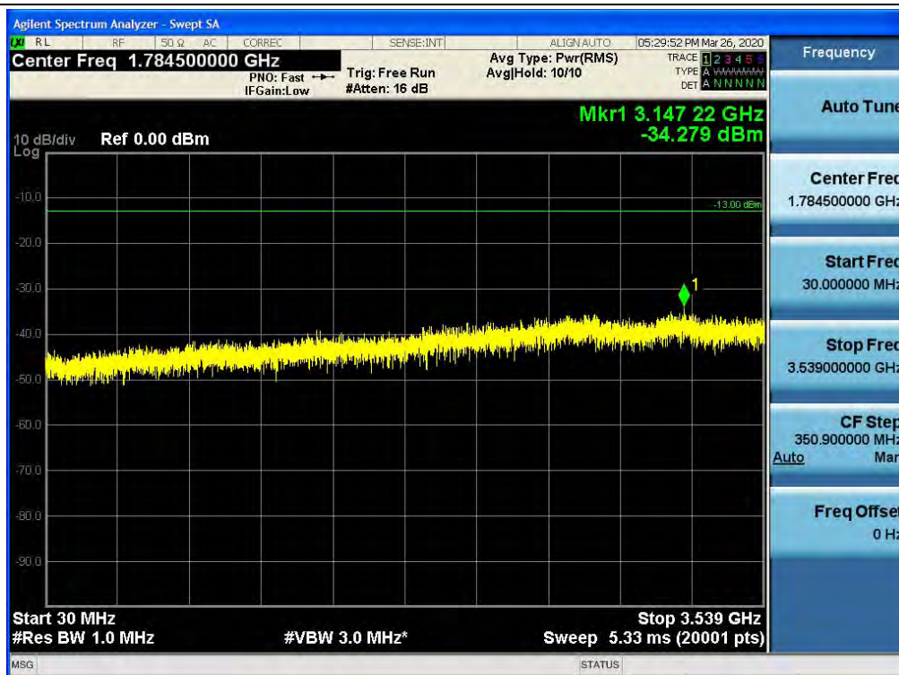
Spurious / CBRS / Downlink / 5G NR 80M / High / 30 MHz ~ Low Edge-10
