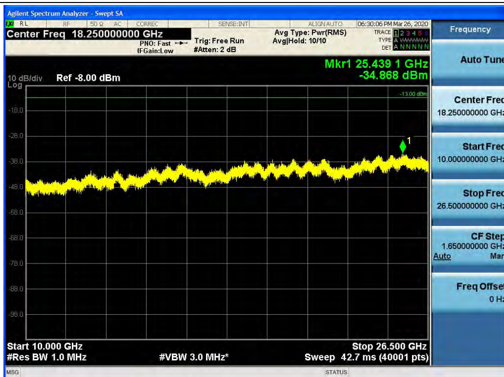
Spurious / CBRS / Downlink / LTE 20 MHz / High / 10 GHz ~ 26.5 GHz
