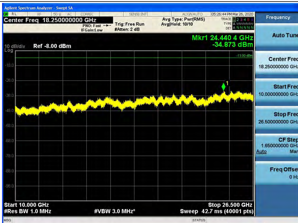
Spurious / CBRS / Downlink / 5G NR 80M / Low / 10 GHz ~ 26.5 GHz
