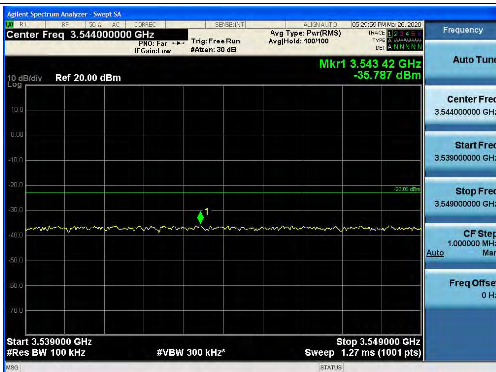
Spurious / CBRS / Downlink / 5G NR 80M / High / Low Edge-10 ~ Low Edge
