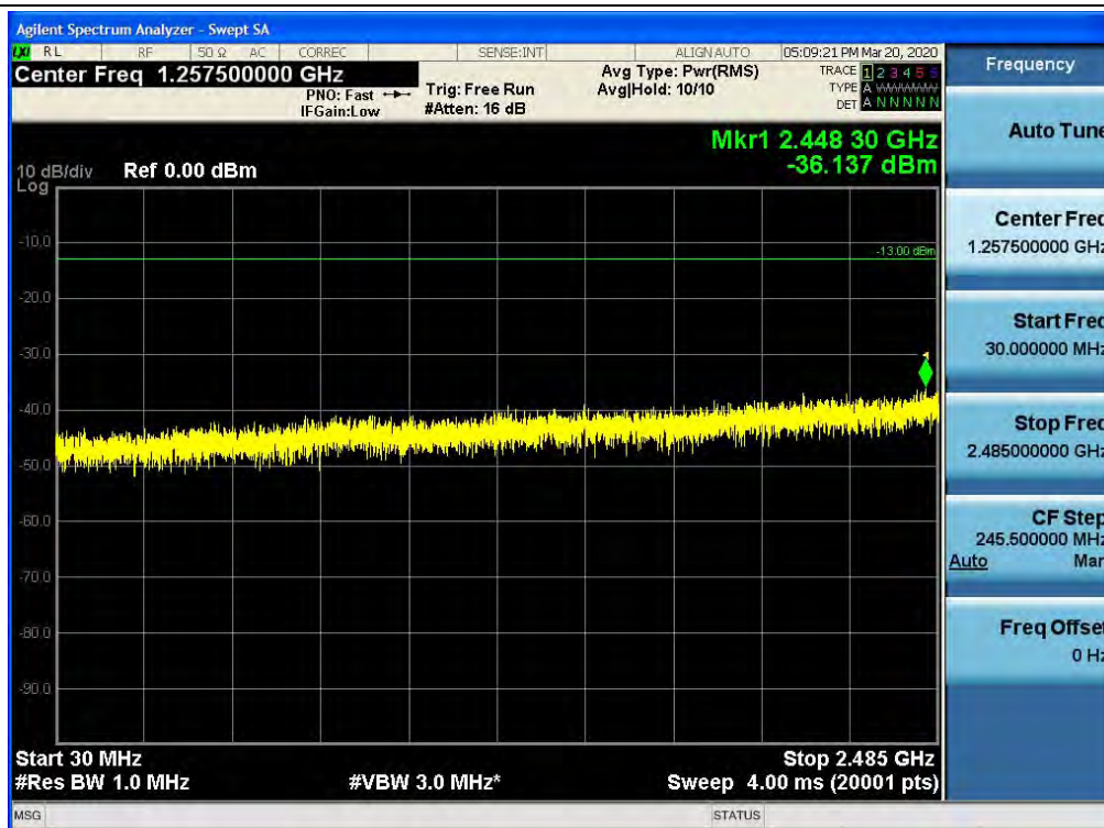
Spurious / BRS/EBS / Downlink / 5G NR 80M / Middle / 30 MHz ~ Low Edge-10
