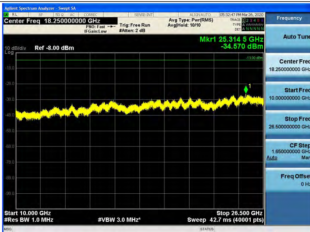
Spurious / CBRS / Downlink / 5G NR 80M / Middle / 10 GHz ~ 26.5 GHz
