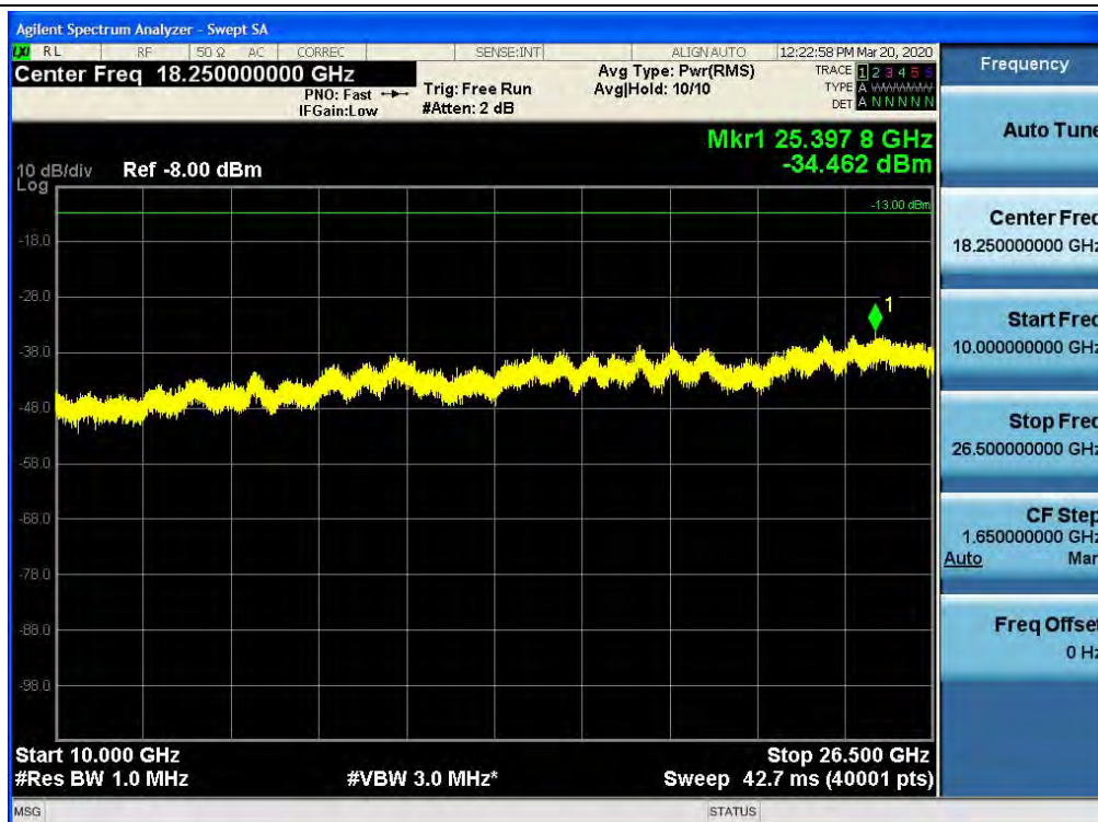
Spurious / Broadband PCS / Downlink / LTE 20 MHz / Middle / 10 GHz ~ 26.5 GHz
