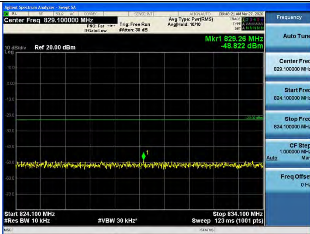
Spurious / ESMR / Uplink / LTE 5 MHz / High / High Edge ~ High Edge+10
