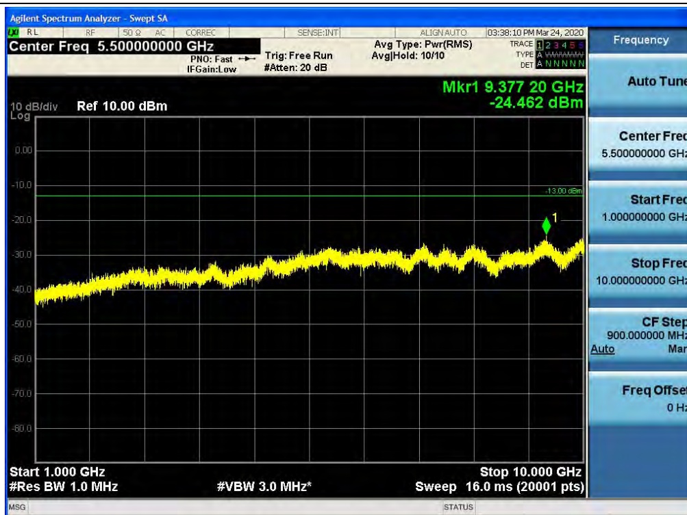
Spurious / Cellular / Uplink / LTE 20 MHz / Low / 1 GHz ~ 10 GHz
