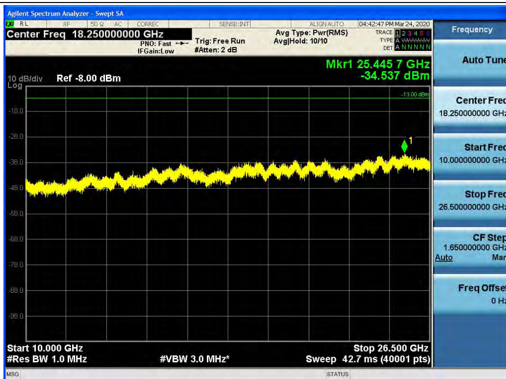
Spurious / Broadband PCS / Uplink / LTE 20 MHz / High / 10 GHz ~ 26.5 GHz
