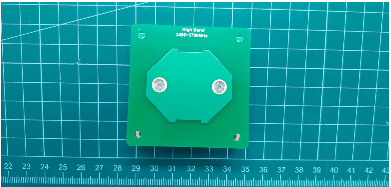
[ADXD-LPR High Band Antenna (top)]
