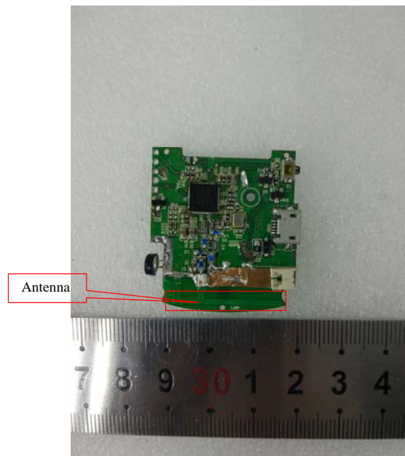
EUT –Main Board Front Shielding off View
