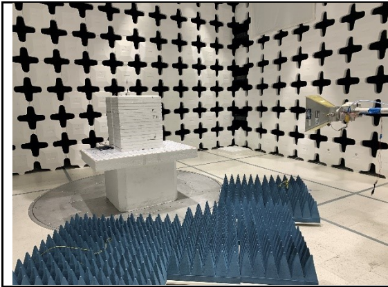
RE above 1GHz test - Front View (Short monopole antenna)
