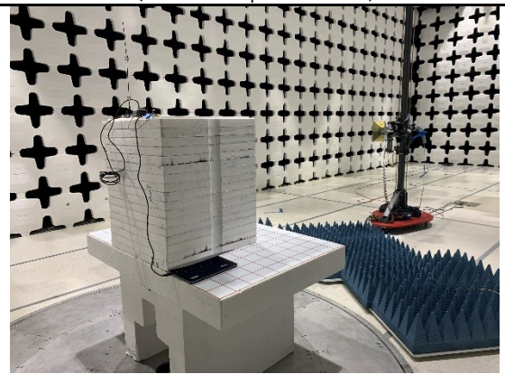
RE above 1GHz test - Rear View (Mag mount antenna)
