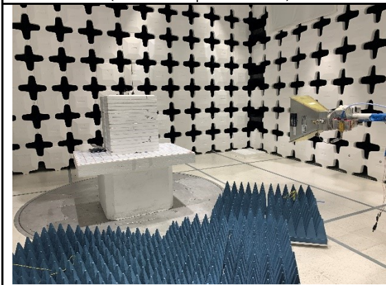
RE above 1GHz test - Front View (Mag mount antenna)
