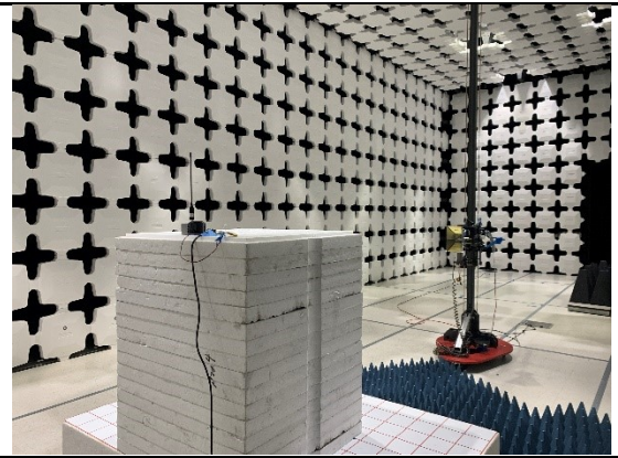
RE above 1GHz test - Rear View (Short monopole antenna)
