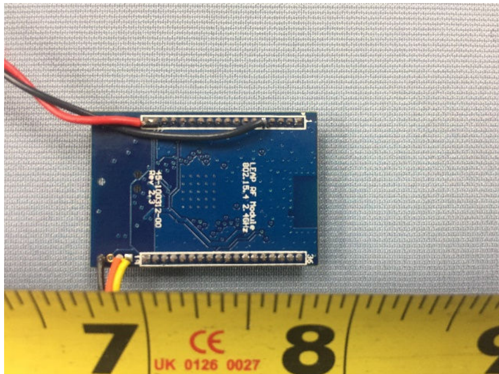
EUT Bottom View – Internal antenna version (44-100312-01)
