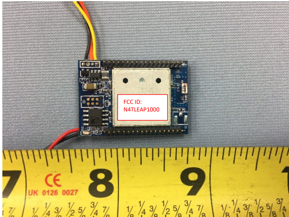
EUT Top View – Internal antenna version (44-100312-01)
