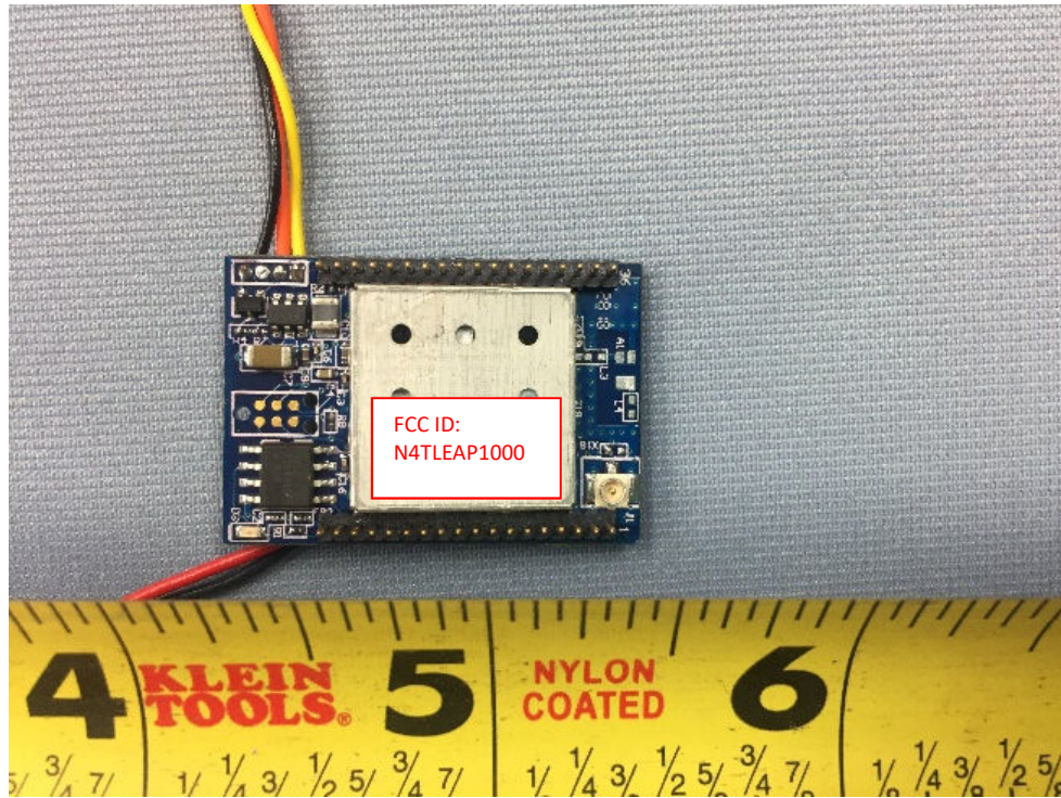
EUT Top View – External antenna version (44-100312-00)
