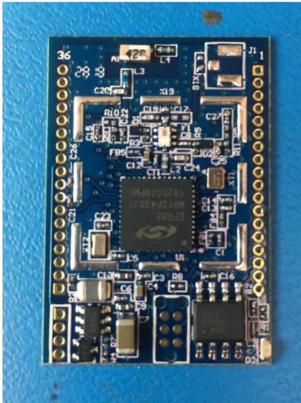
EUT Top View – Internal antenna version
