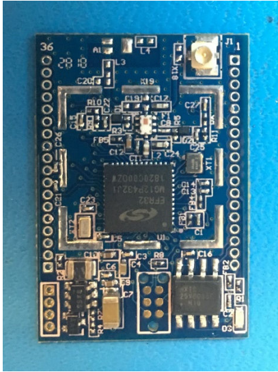
EUT Top View – External antenna version
