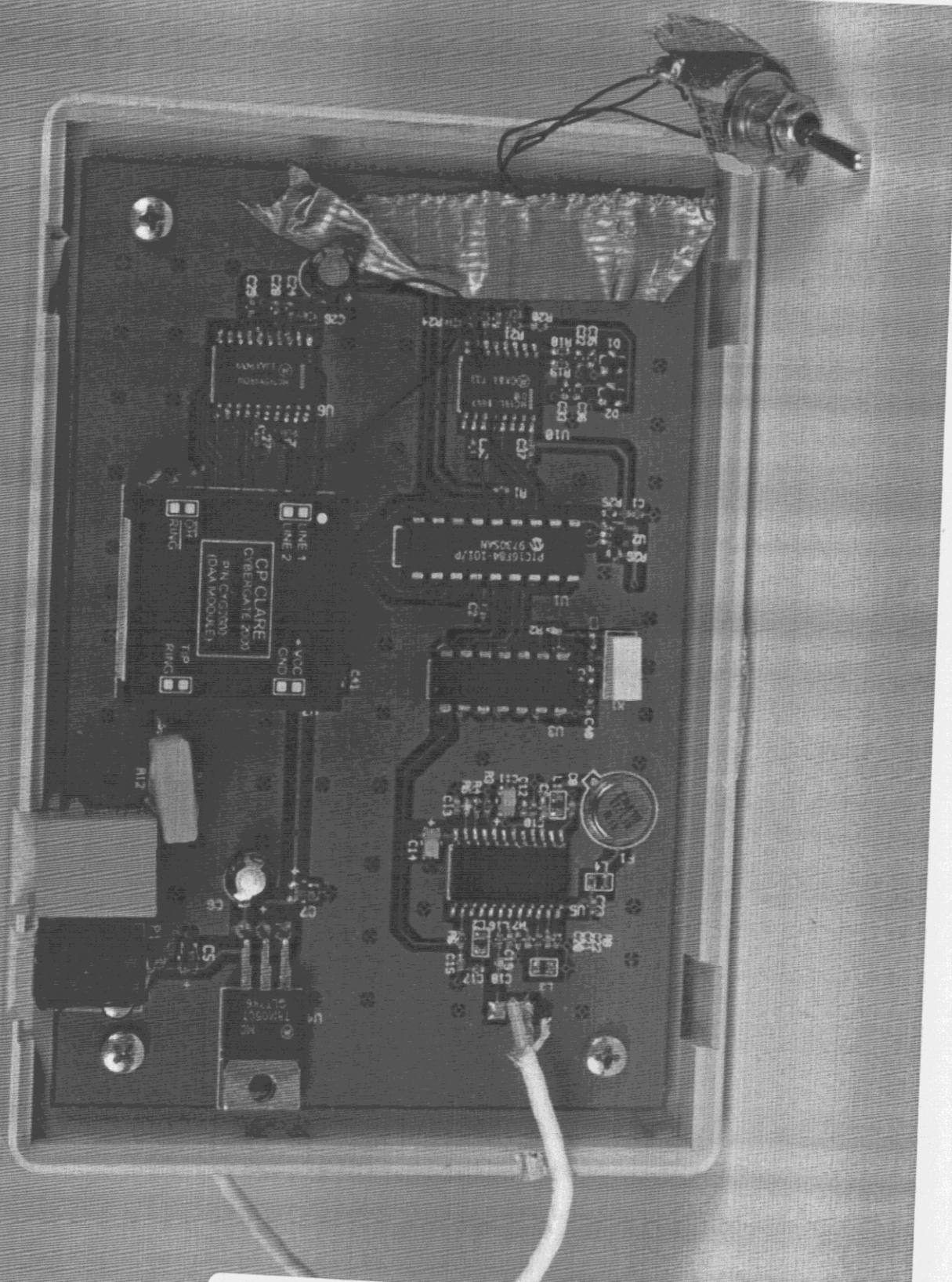
Lectoron Technologies Project no.: 8R00115.2 Model: Lectoron 20 Receiver FCC ID: N48202RECEIVER Component placement
