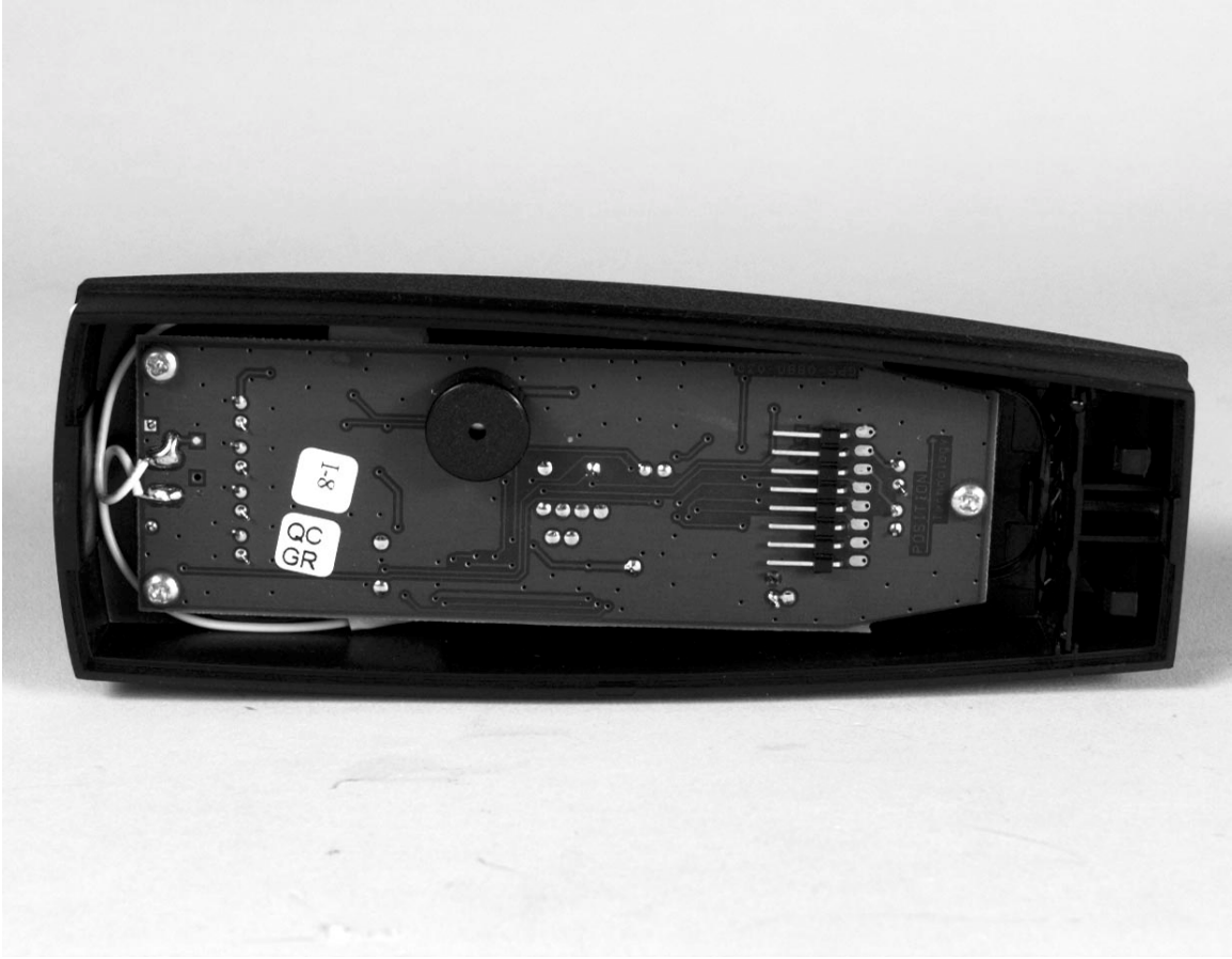
PCB Trace Side
