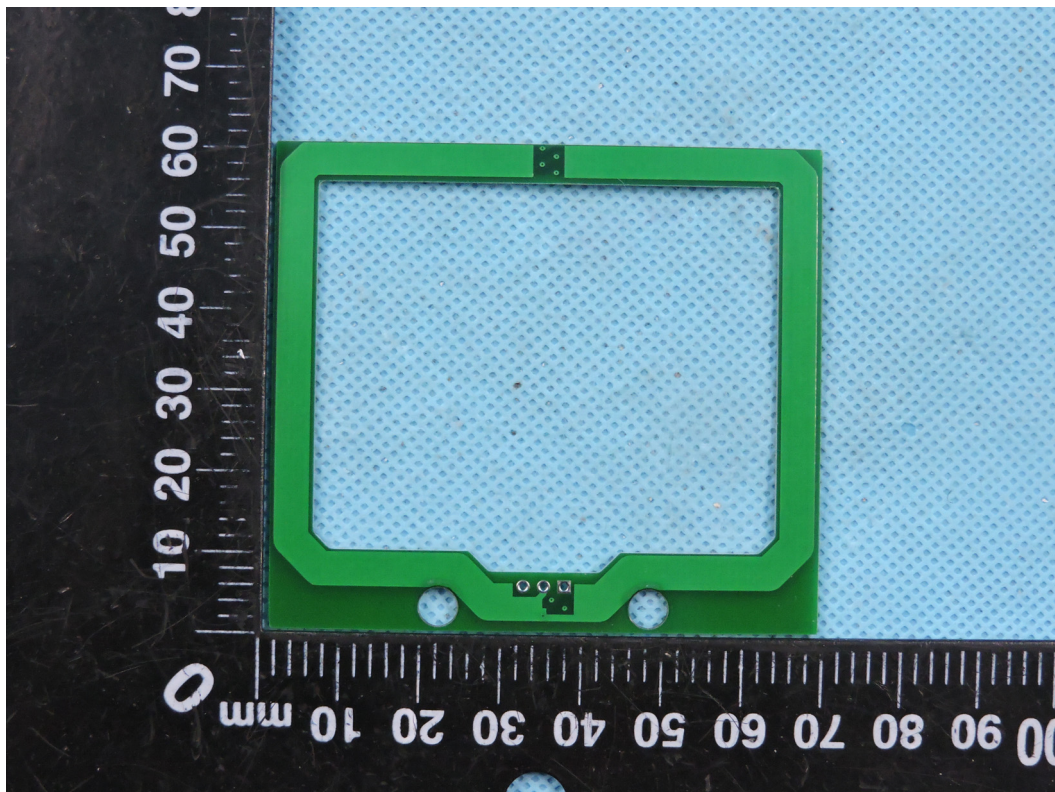
Photo 28 ( NXT-5M )
