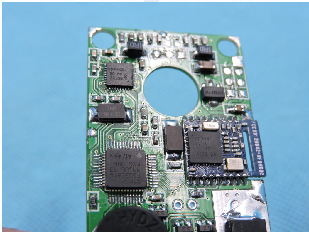
Photo 22 ( NXT-5M )
