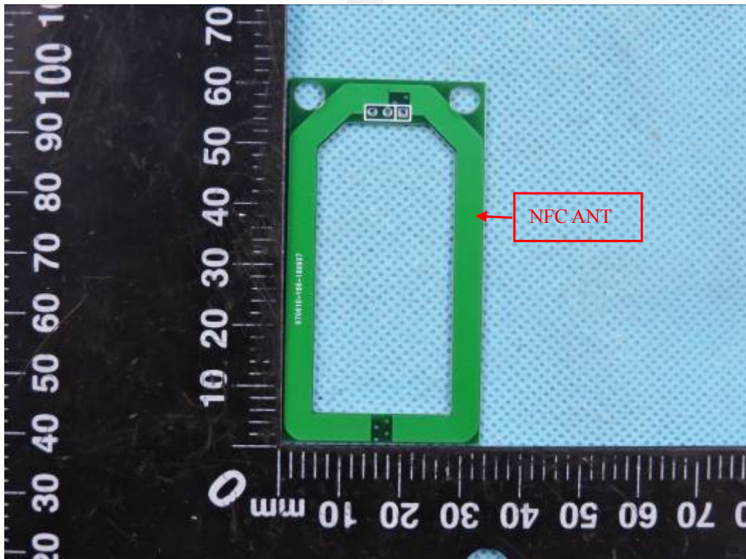
Photo 17 ( NXT-3M )
