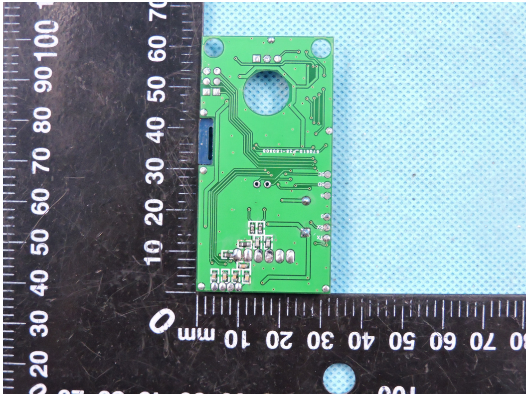
Photo 26 ( NXT-5M )
