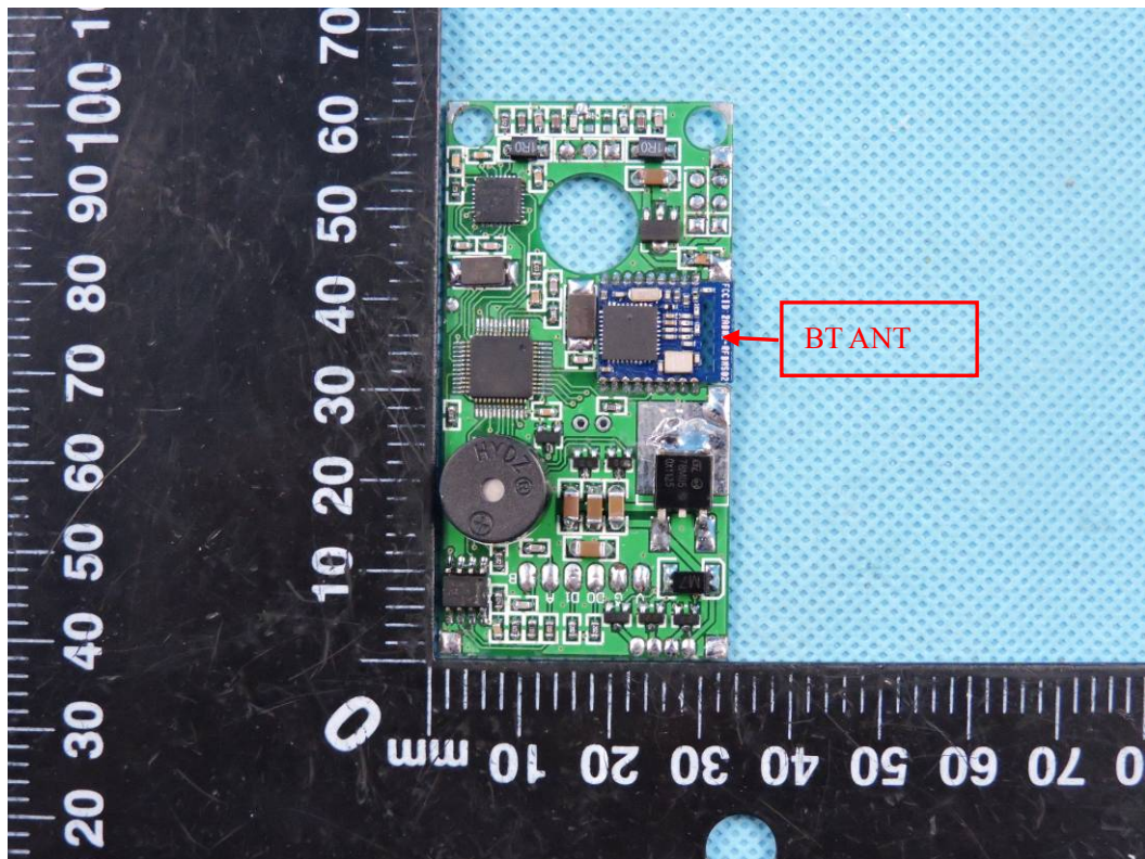
Photo 13 ( NXT-3M )
