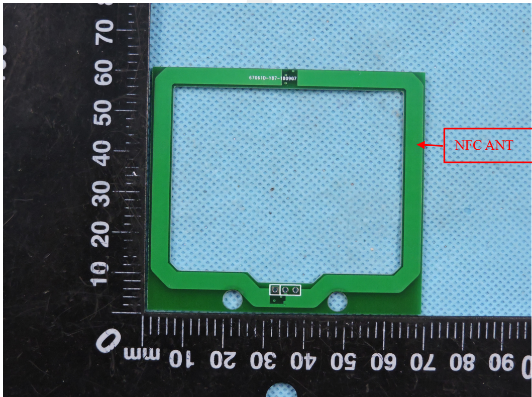
Photo 26 ( NXT-5M )
