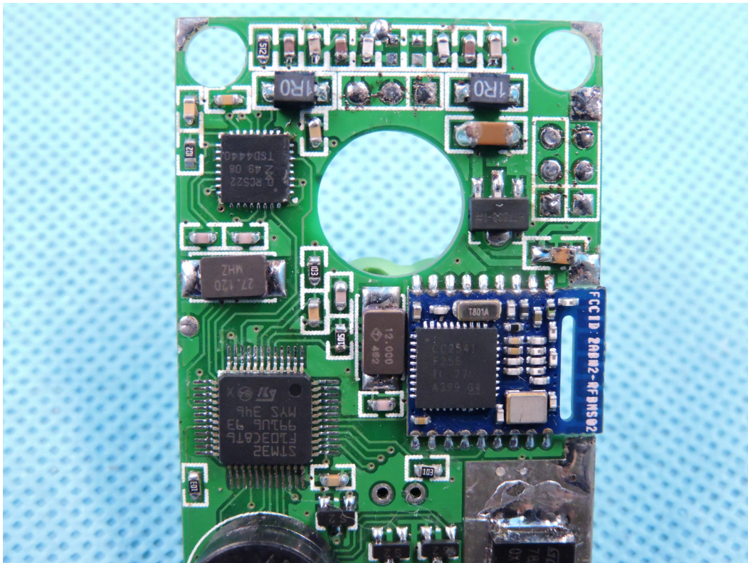
Photo 24 ( NXT-5M )
