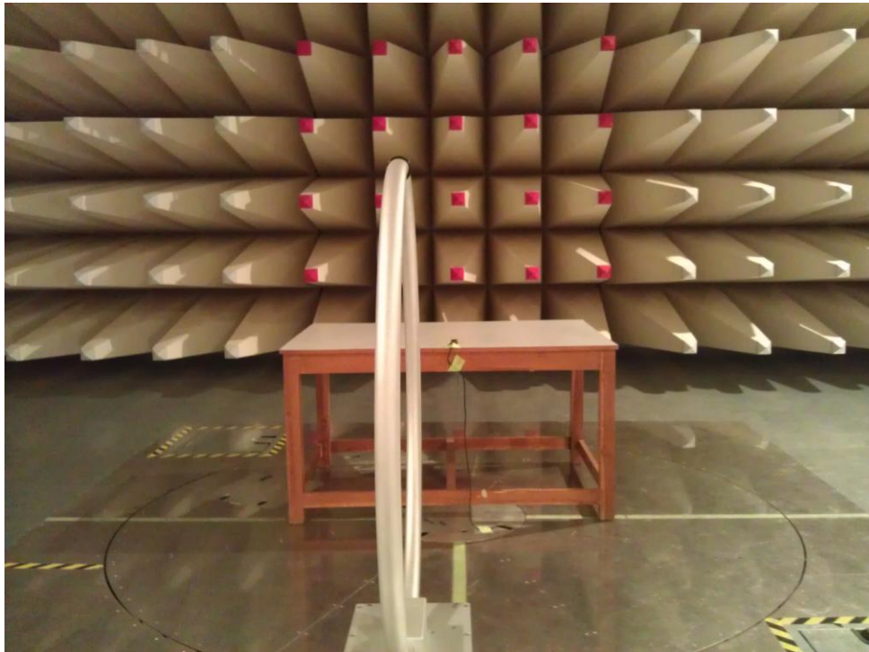
Test setup
