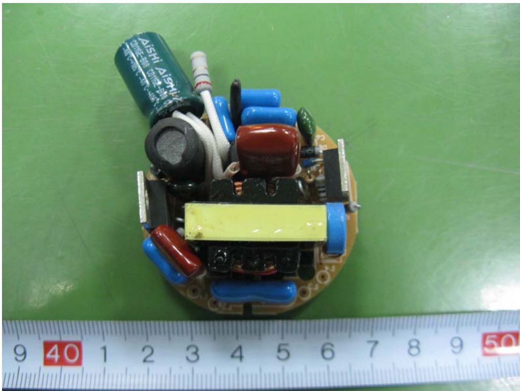
CMTL 30W: EUT – Board Top Assembly Components View
