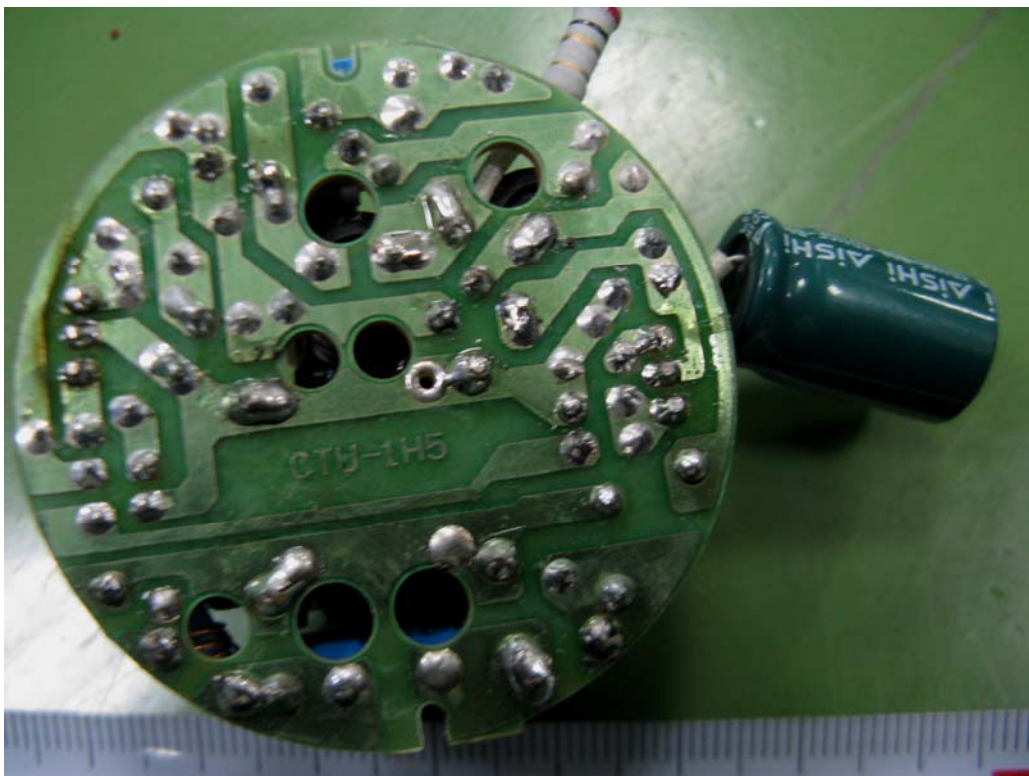
CMTL 25W: EUT – Board Bottom Components View
