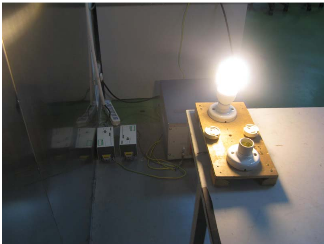
CMTL 25W: Conducted Emissions - Side View
