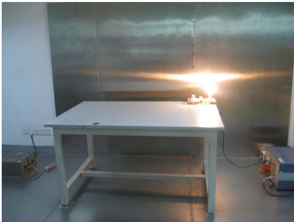
CMTL 30W: Conducted Emissions - Side View
