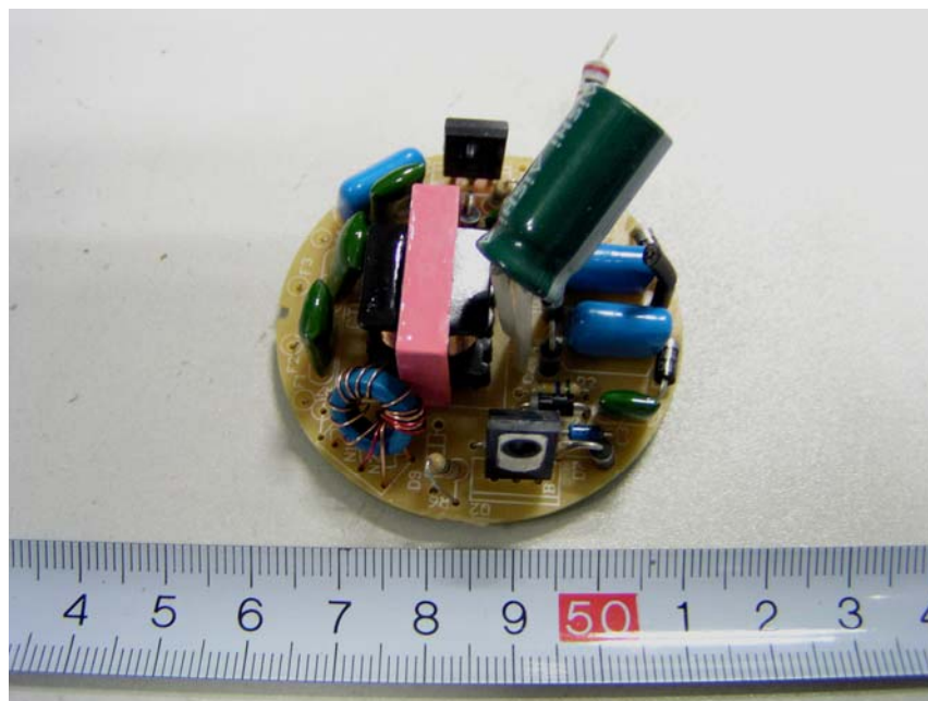
CPTL13W: EUT-PCB View (1)
