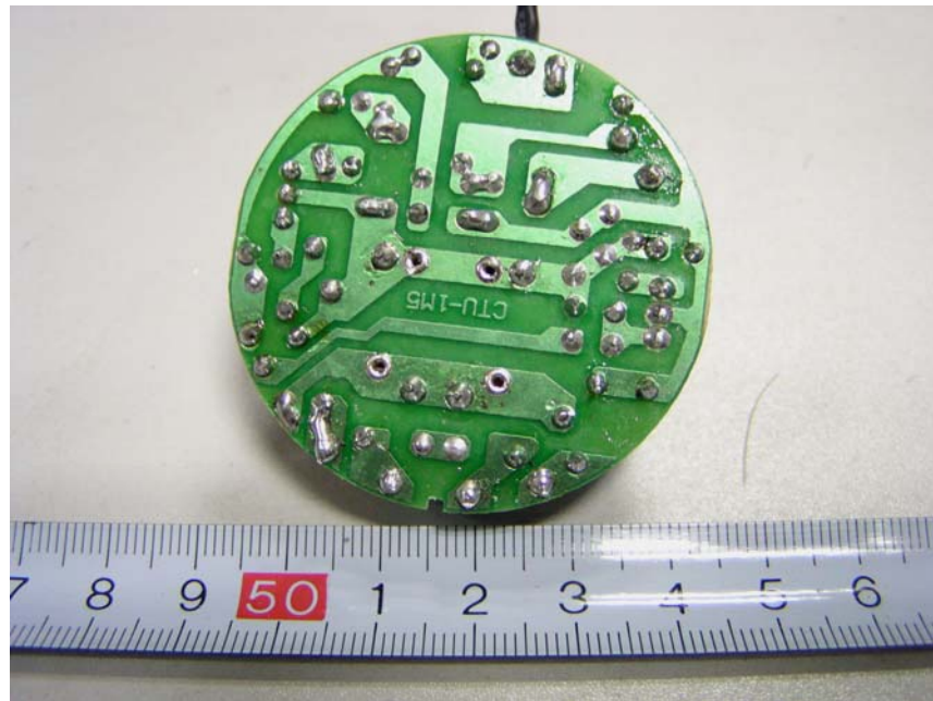
CPTL25W: EUT-PCB View (2)
