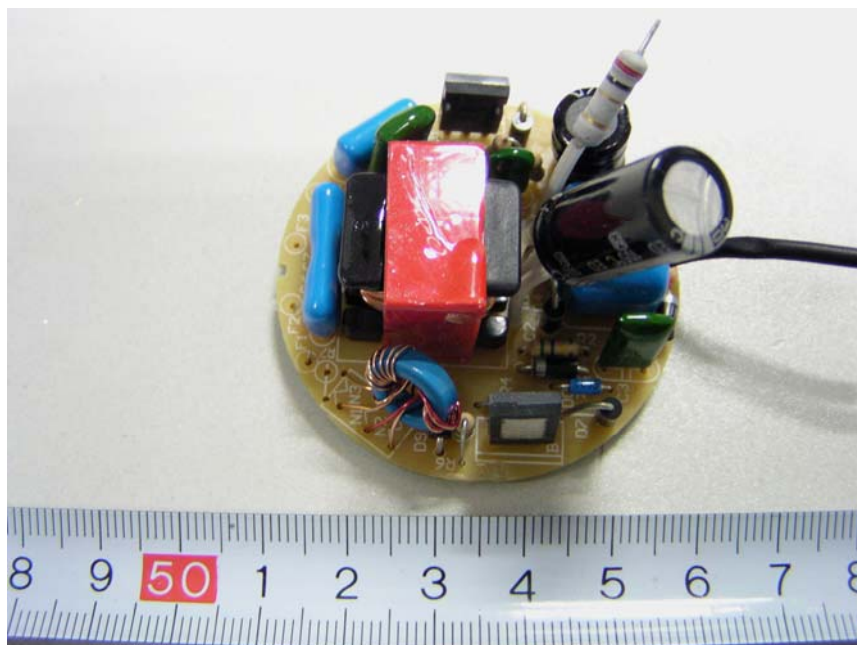
CPTL25W: EUT-PCB View (1)
