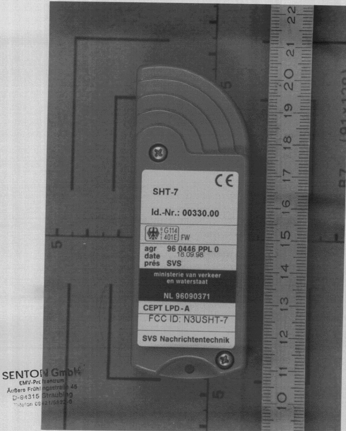
Bottom view of transmitter (with label)
