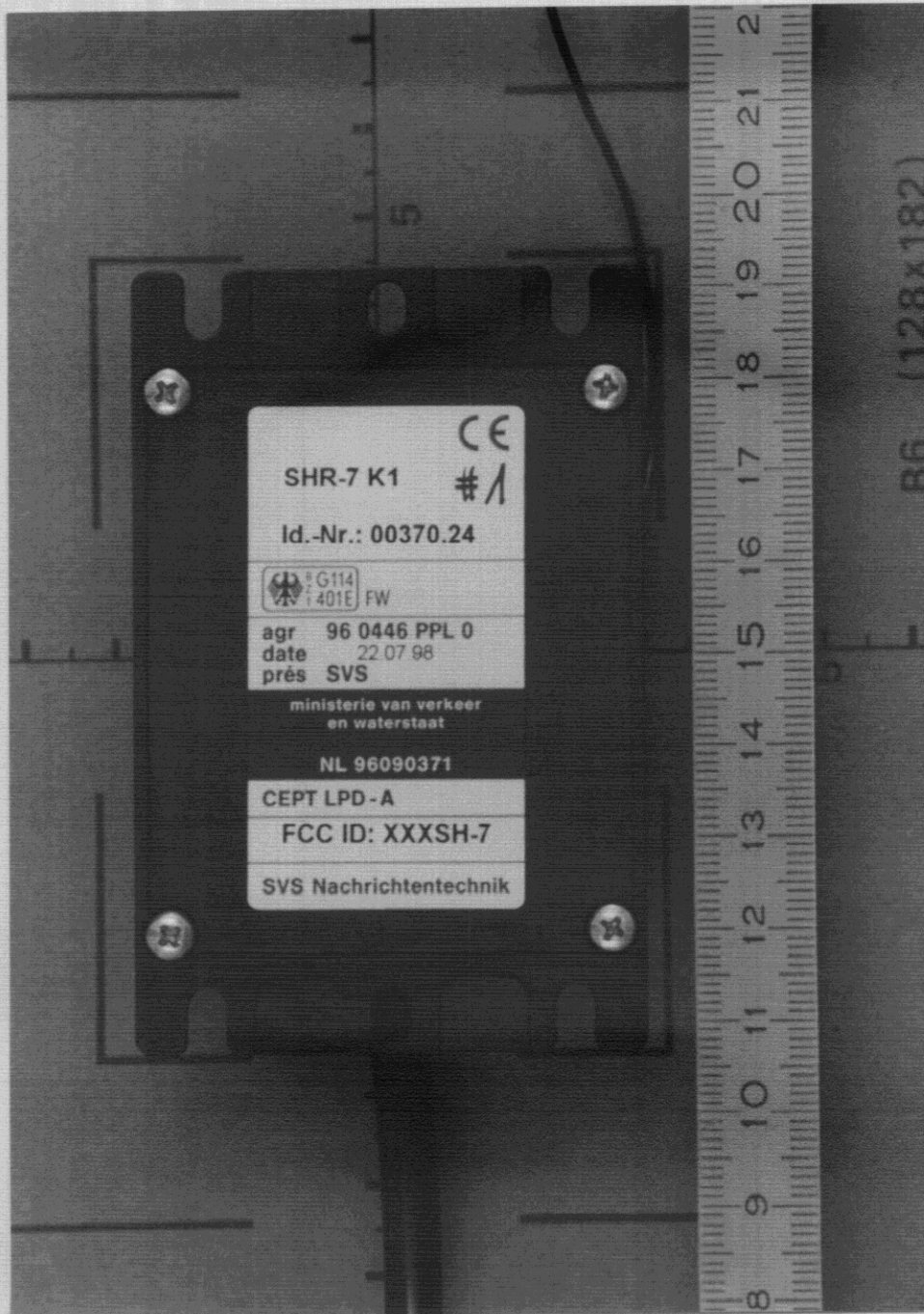
Bottom view of receiver (with label)
