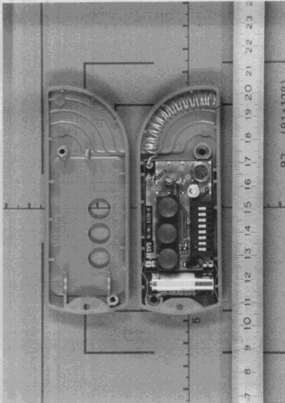
Top view of disassembled transmitter
